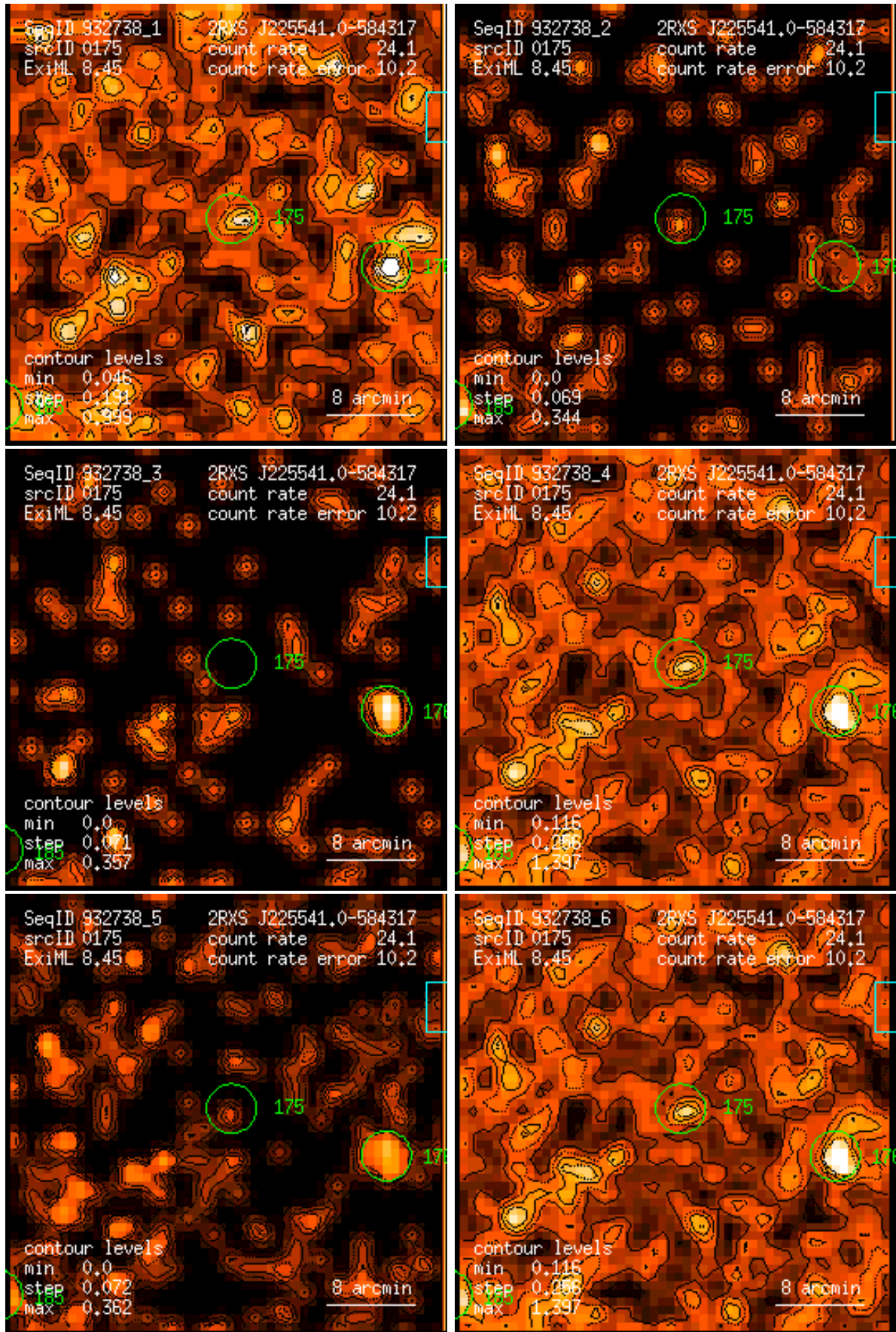
Figure 175: RASS 932738: detection 0175: band rate images, Gaussian filter: (1) PSPC channels 11 – 41, (2) 52 – 90, (3) 91 – 201, (4) 11 – 235, (5) 52 – 201, (6) 11 – 201. Broad band rates in counts/ks. Band rate contour levels in counts/ks/arcmin 2 .
