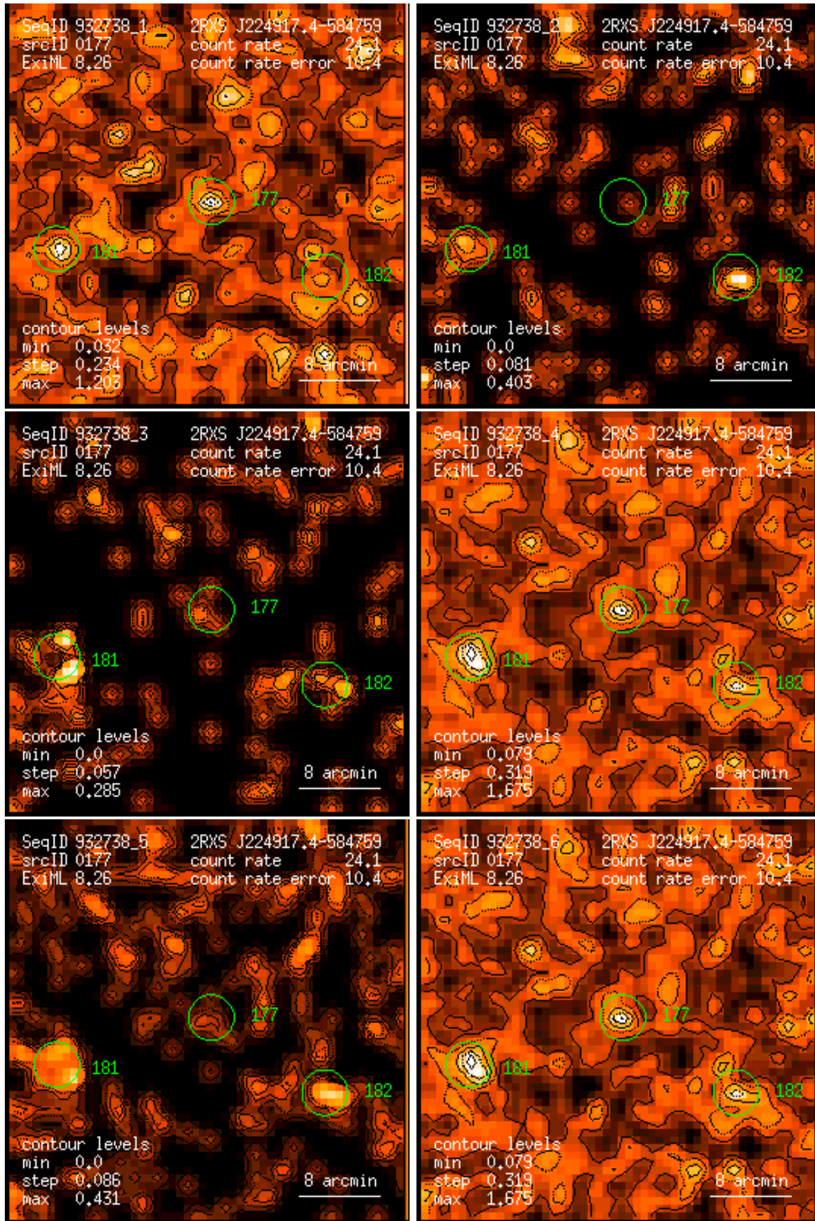
Figure 177: RASS 932738: detection 0177: band rate images, Gaussian filter: (1) PSPC channels 11 – 41, (2) 52 – 90, (3) 91 – 201, (4) 11 – 235, (5) 52 – 201, (6) 11 – 201. Broad band rates in counts/ks. Band rate contour levels in counts/ks/arcmin 2 .
