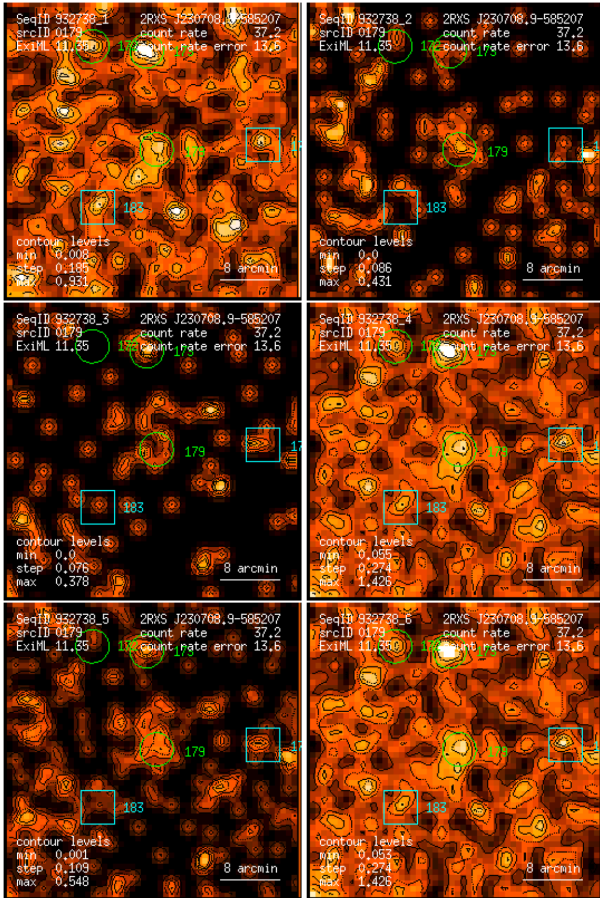
Figure 179: RASS 932738: detection 0179: band rate images, Gaussian filter: (1) PSPC channels 11 – 41, (2) 52 – 90, (3) 91 – 201, (4) 11 – 235, (5) 52 – 201, (6) 11 – 201. Broad band rates in counts/ks. Band rate contour levels in counts/ks/arcmin 2 .
