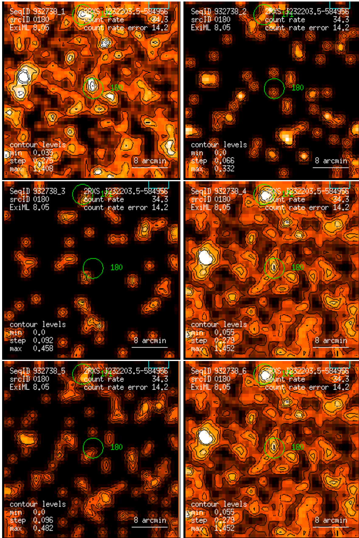
Figure 180: RASS 932738: detection 0180: band rate images, Gaussian filter: (1) PSPC channels 11 – 41, (2) 52 – 90, (3) 91 – 201, (4) 11 – 235, (5) 52 – 201, (6) 11 – 201. Broad band rates in counts/ks. Band rate contour levels in counts/ks/arcmin 2 .
