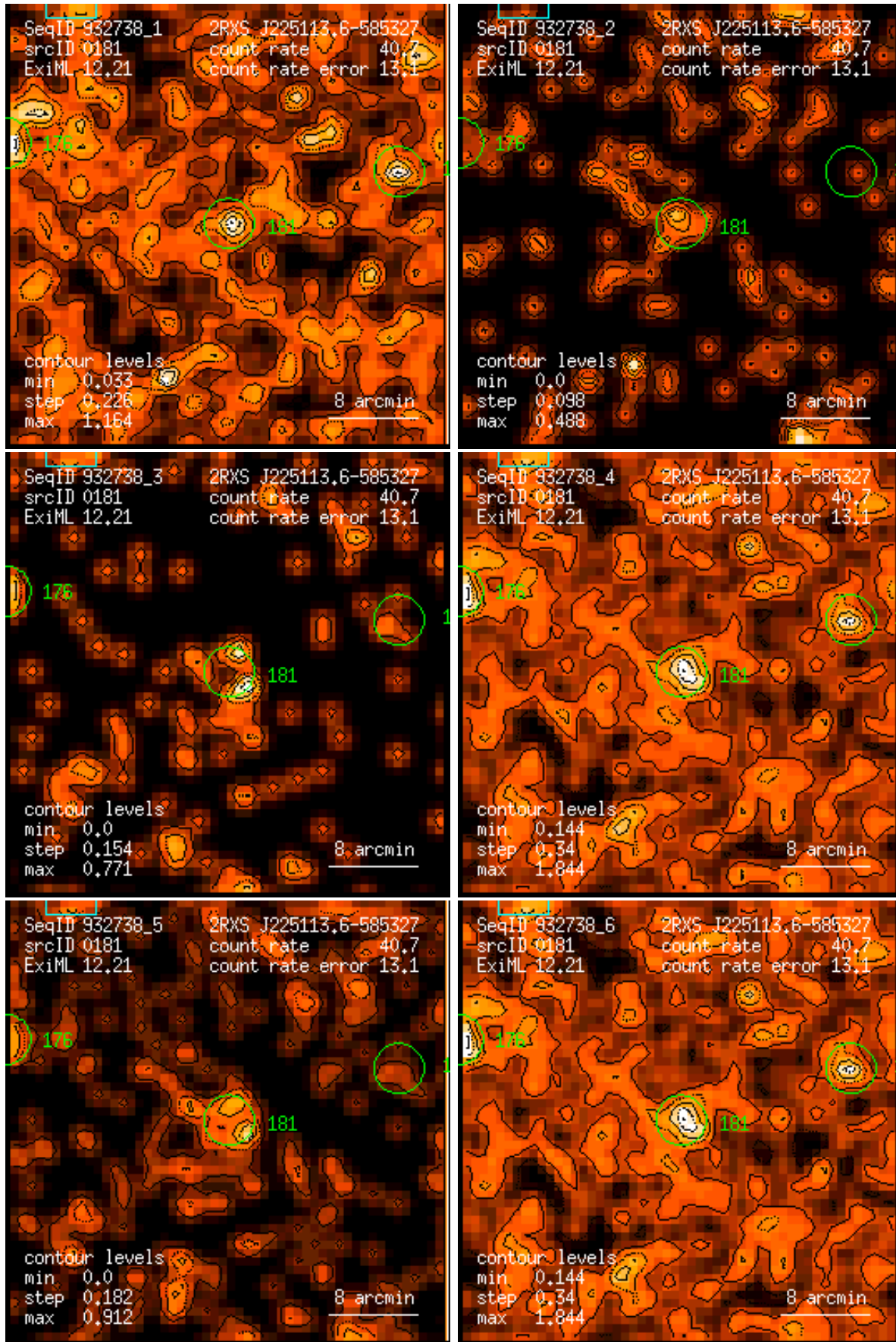
Figure 181: RASS 932738: detection 0181: band rate images, Gaussian filter: (1) PSPC channels 11 – 41, (2) 52 – 90, (3) 91 – 201, (4) 11 – 235, (5) 52 – 201, (6) 11 – 201. Broad band rates in counts/ks. Band rate contour levels in counts/ks/arcmin 2 .
