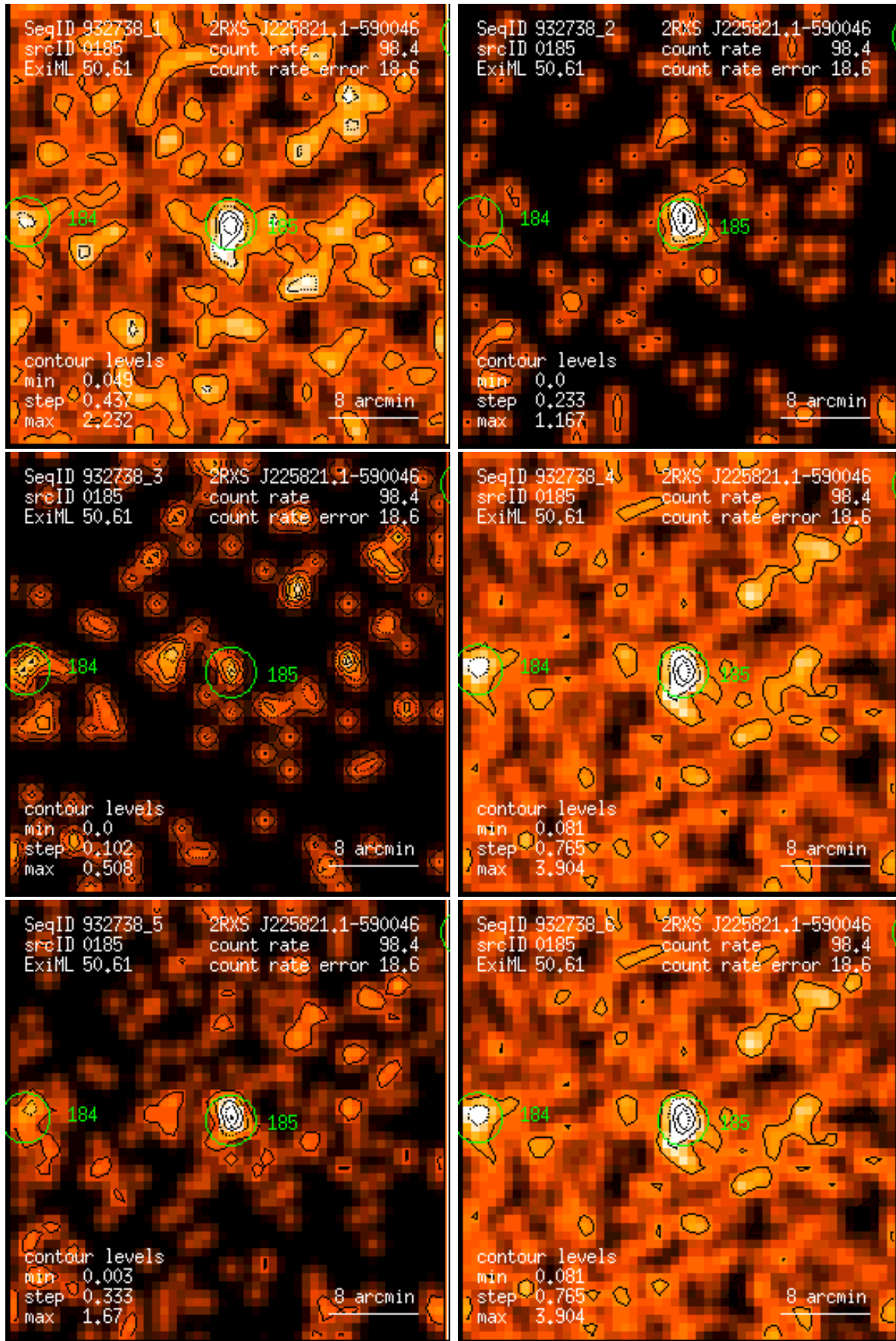
Figure 185: RASS 932738: detection 0185: band rate images, Gaussian filter: (1) PSPC channels 11 – 41, (2) 52 – 90, (3) 91 – 201, (4) 11 – 235, (5) 52 – 201, (6) 11 – 201. Broad band rates in counts/ks. Band rate contour levels in counts/ks/arcmin 2 .
