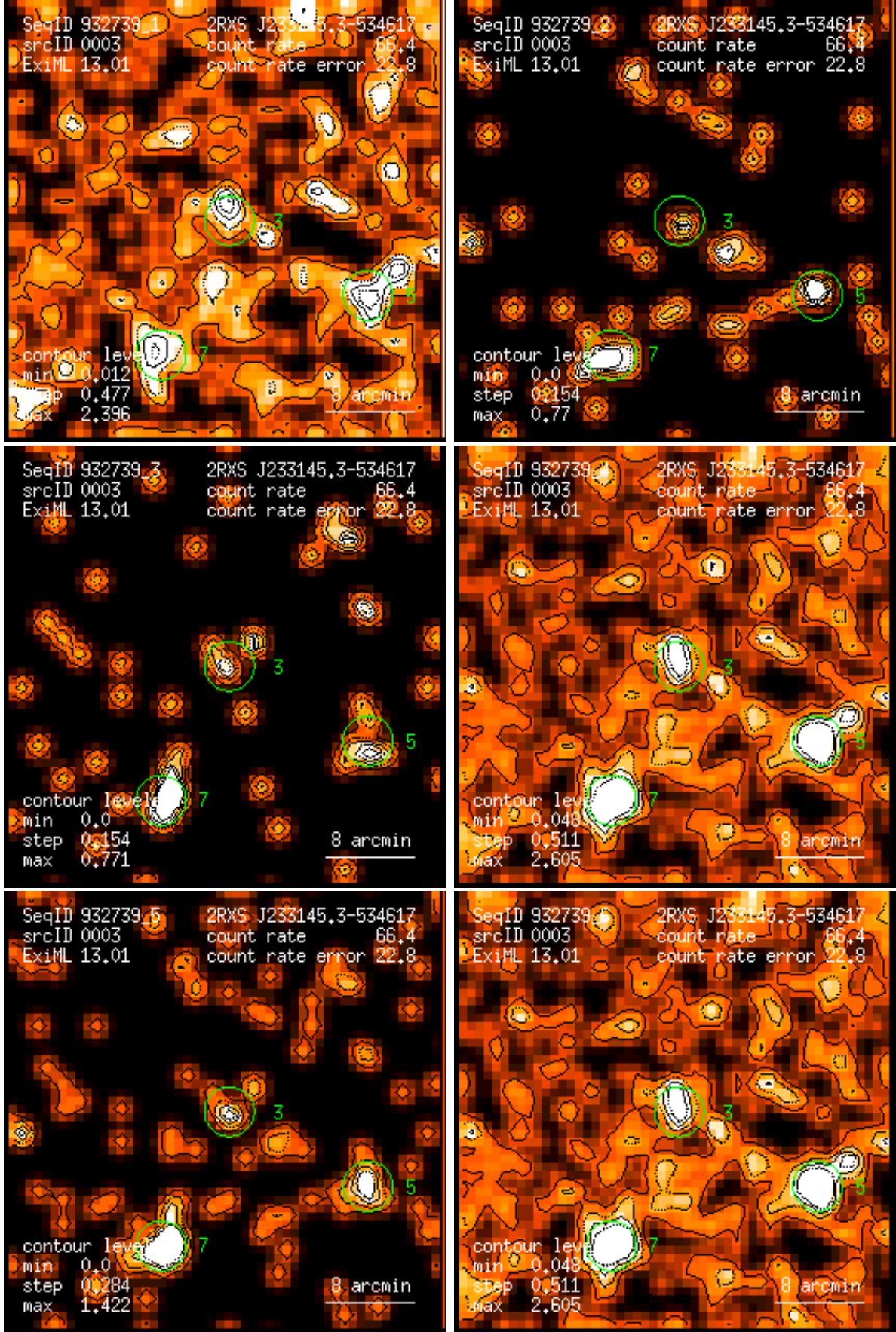
Figure 3: RASS 932739: detection 0003: band rate images, Gaussian filter: (1) PSPC channels 11 – 41, (2) 52 – 90, (3) 91 – 201, (4) 11 – 235, (5) 52 – 201, (6) 11 – 201. Broad band rates in counts/ks. Band rate contour levels in counts/ks/arcmin 2 .
