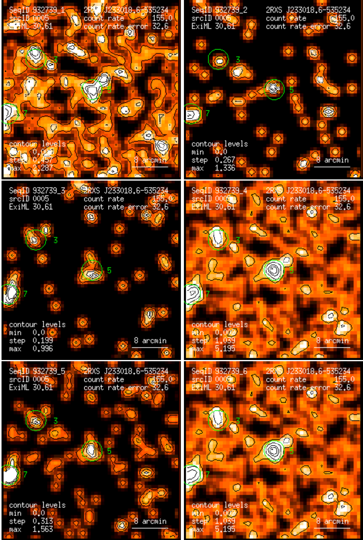
Figure 5: RASS 932739: detection 0005: band rate images, Gaussian filter: (1) PSPC channels 11 – 41, (2) 52 – 90, (3) 91 – 201, (4) 11 – 235, (5) 52 – 201, (6) 11 – 201. Broad band rates in counts/ks. Band rate contour levels in counts/ks/arcmin 2 .
