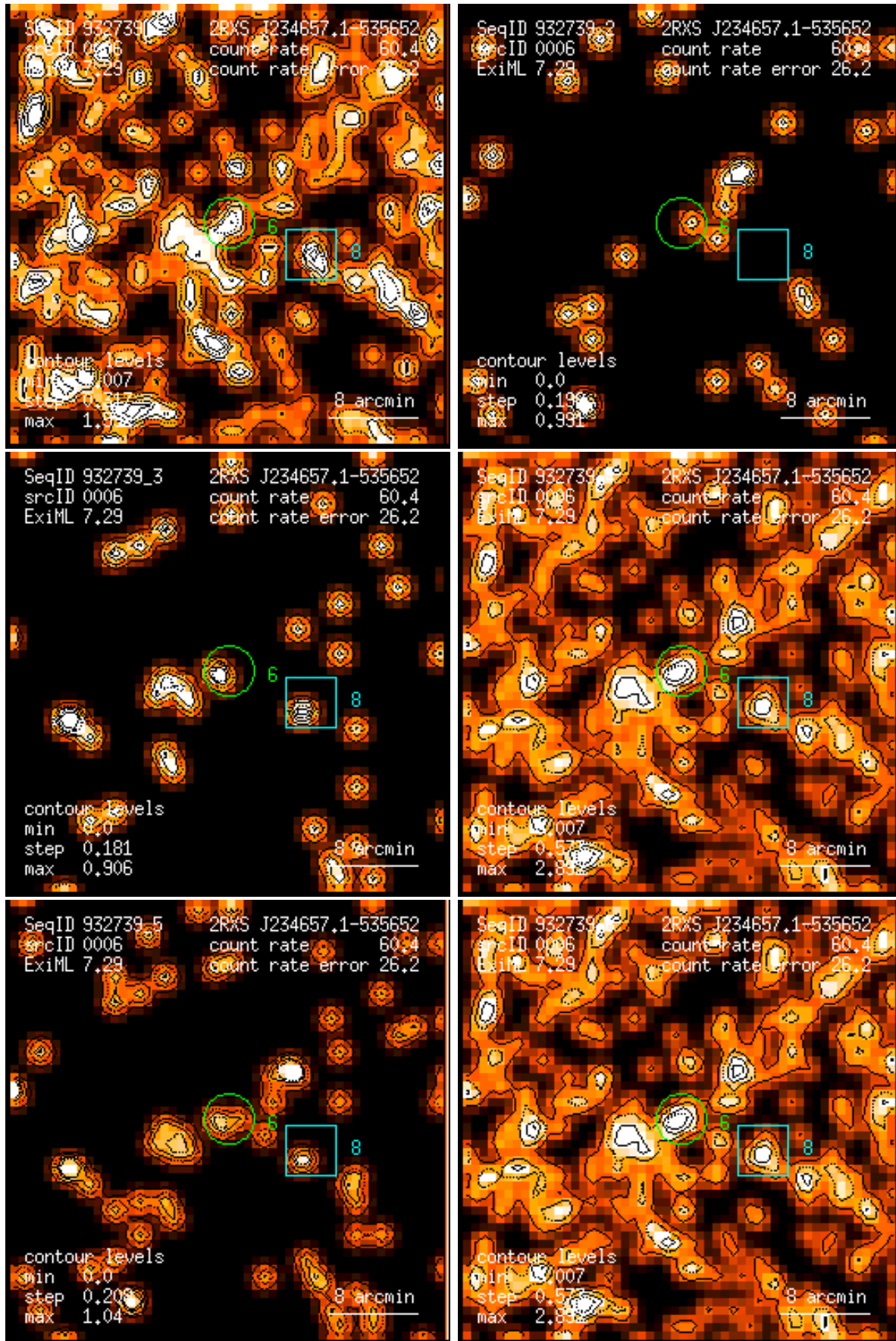
Figure 6: RASS 932739: detection 0006: band rate images, Gaussian filter: (1) PSPC channels 11 – 41, (2) 52 – 90, (3) 91 – 201, (4) 11 – 235, (5) 52 – 201, (6) 11 – 201. Broad band rates in counts/ks. Band rate contour levels in counts/ks/arcmin 2 .
