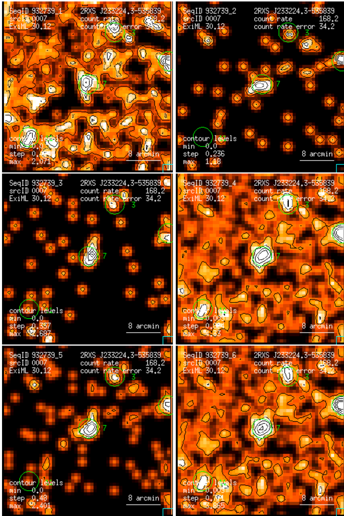
Figure 7: RASS 932739: detection 0007: band rate images, Gaussian filter: (1) PSPC channels 11 – 41, (2) 52 – 90, (3) 91 – 201, (4) 11 – 235, (5) 52 – 201, (6) 11 – 201. Broad band rates in counts/ks. Band rate contour levels in counts/ks/arcmin 2 .
