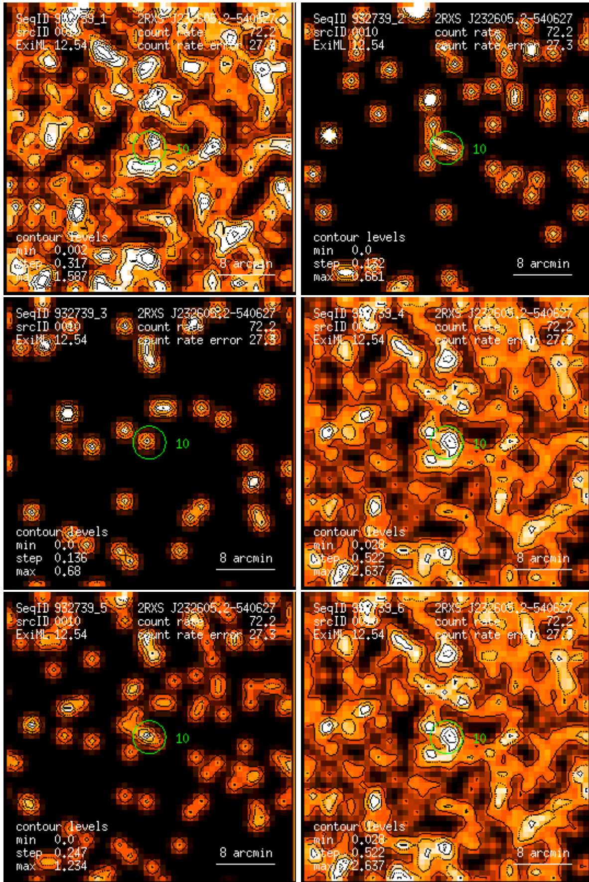
Figure 10: RASS 932739: detection 0010: band rate images, Gaussian filter: (1) PSPC channels 11 – 41, (2) 52 – 90, (3) 91 – 201, (4) 11 – 235, (5) 52 – 201, (6) 11 – 201. Broad band rates in counts/ks. Band rate contour levels in counts/ks/arcmin 2 .
