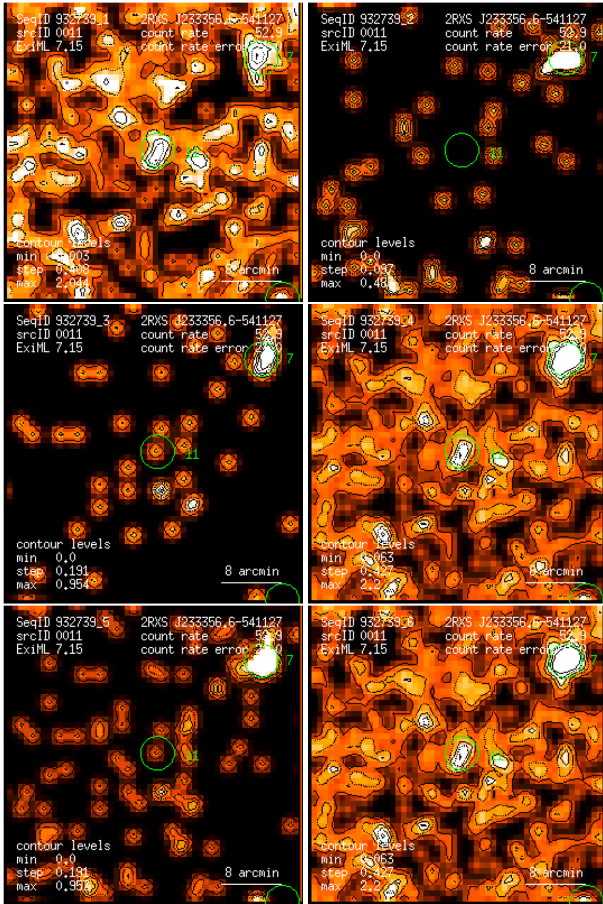
Figure 11: RASS 932739: detection 0011: band rate images, Gaussian filter: (1) PSPC channels 11 – 41, (2) 52 – 90, (3) 91 – 201, (4) 11 – 235, (5) 52 – 201, (6) 11 – 201. Broad band rates in counts/ks. Band rate contour levels in counts/ks/arcmin 2 .
