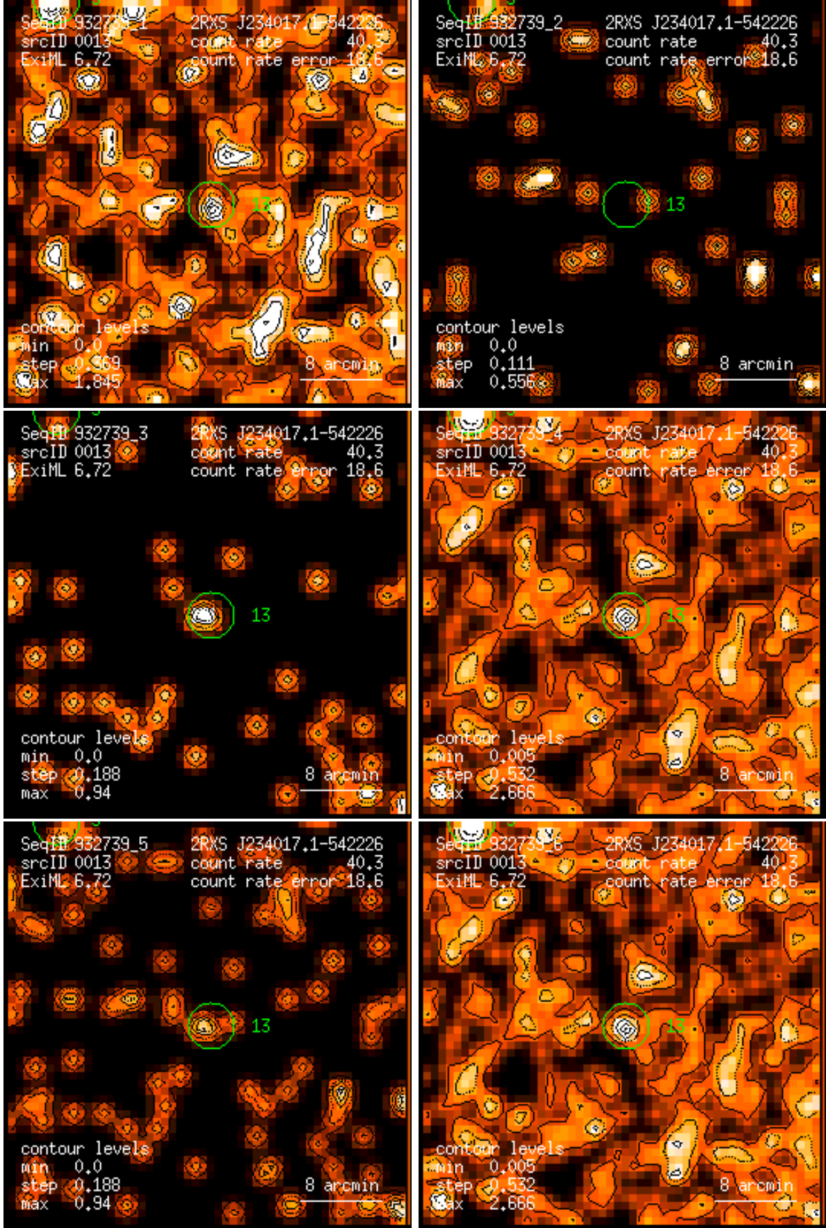
Figure 13: RASS 932739: detection 0013: band rate images, Gaussian filter: (1) PSPC channels 11 – 41, (2) 52 – 90, (3) 91 – 201, (4) 11 – 235, (5) 52 – 201, (6) 11 – 201. Broad band rates in counts/ks. Band rate contour levels in counts/ks/arcmin 2 .
