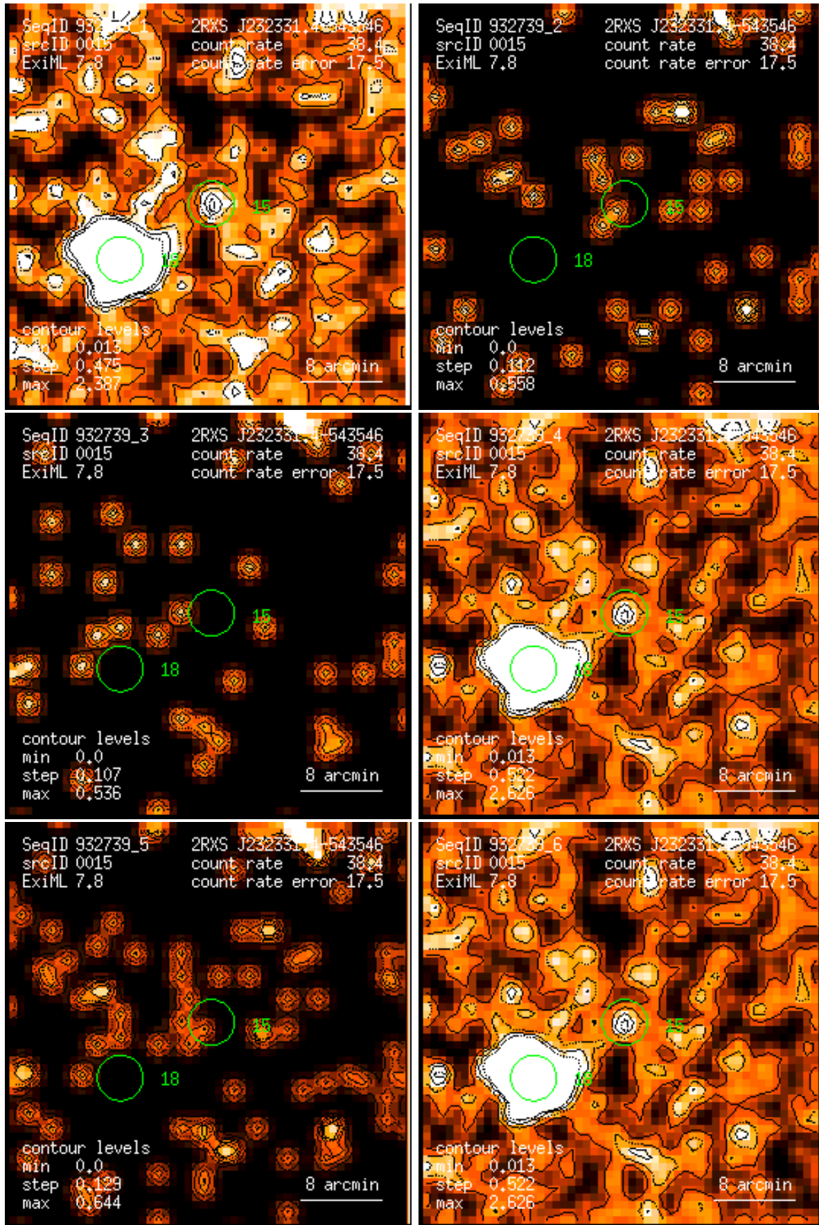
Figure 15: RASS 932739: detection 0015: band rate images, Gaussian filter: (1) PSPC channels 11 – 41, (2) 52 – 90, (3) 91 – 201, (4) 11 – 235, (5) 52 – 201, (6) 11 – 201. Broad band rates in counts/ks. Band rate contour levels in counts/ks/arcmin 2 .
