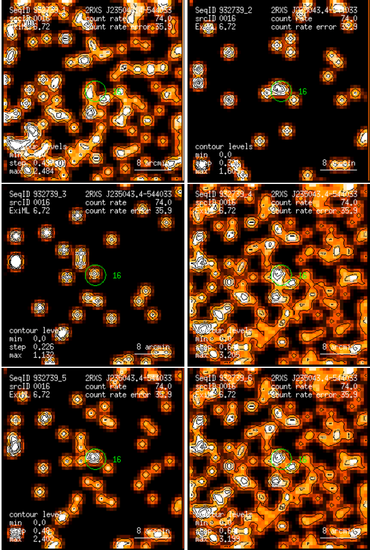
Figure 16: RASS 932739: detection 0016: band rate images, Gaussian filter: (1) PSPC channels 11 – 41, (2) 52 – 90, (3) 91 – 201, (4) 11 – 235, (5) 52 – 201, (6) 11 – 201. Broad band rates in counts/ks. Band rate contour levels in counts/ks/arcmin 2 .
