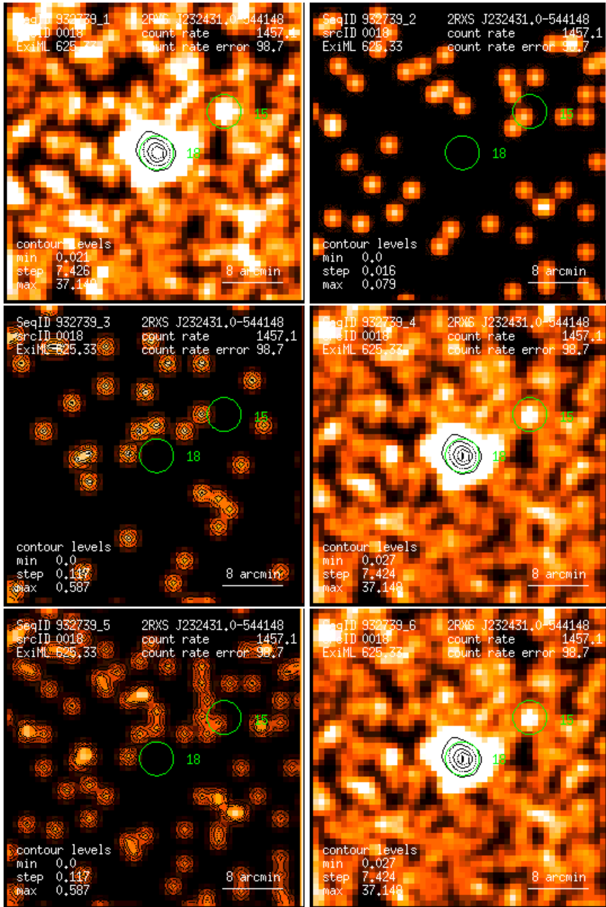
Figure 18: RASS 932739: detection 0018: band rate images, Gaussian filter: (1) PSPC channels 11 – 41, (2) 52 – 90, (3) 91 – 201, (4) 11 – 235, (5) 52 – 201, (6) 11 – 201. Broad band rates in counts/ks. Band rate contour levels in counts/ks/arcmin 2 .
