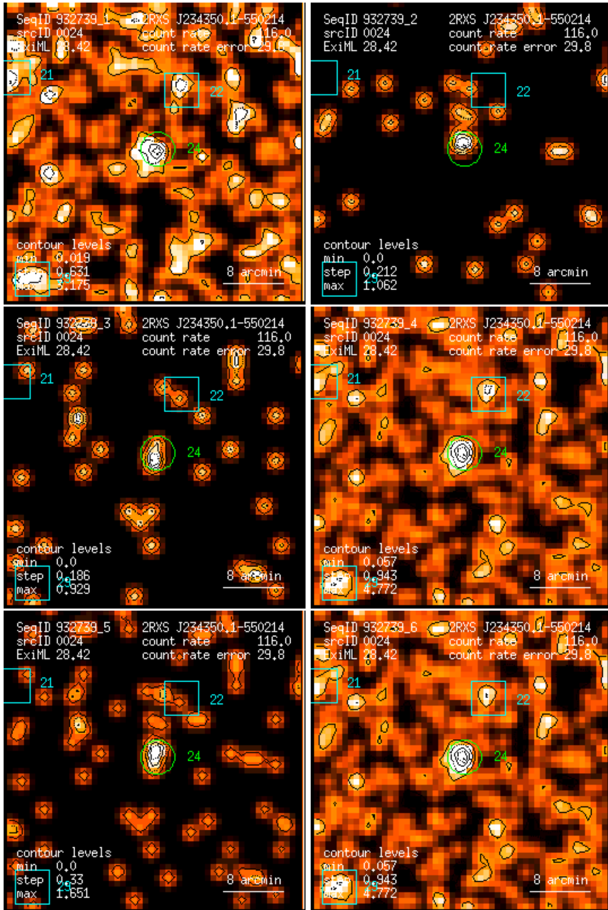
Figure 24: RASS 932739: detection 0024: band rate images, Gaussian filter: (1) PSPC channels 11 – 41, (2) 52 – 90, (3) 91 – 201, (4) 11 – 235, (5) 52 – 201, (6) 11 – 201. Broad band rates in counts/ks. Band rate contour levels in counts/ks/arcmin 2 .
