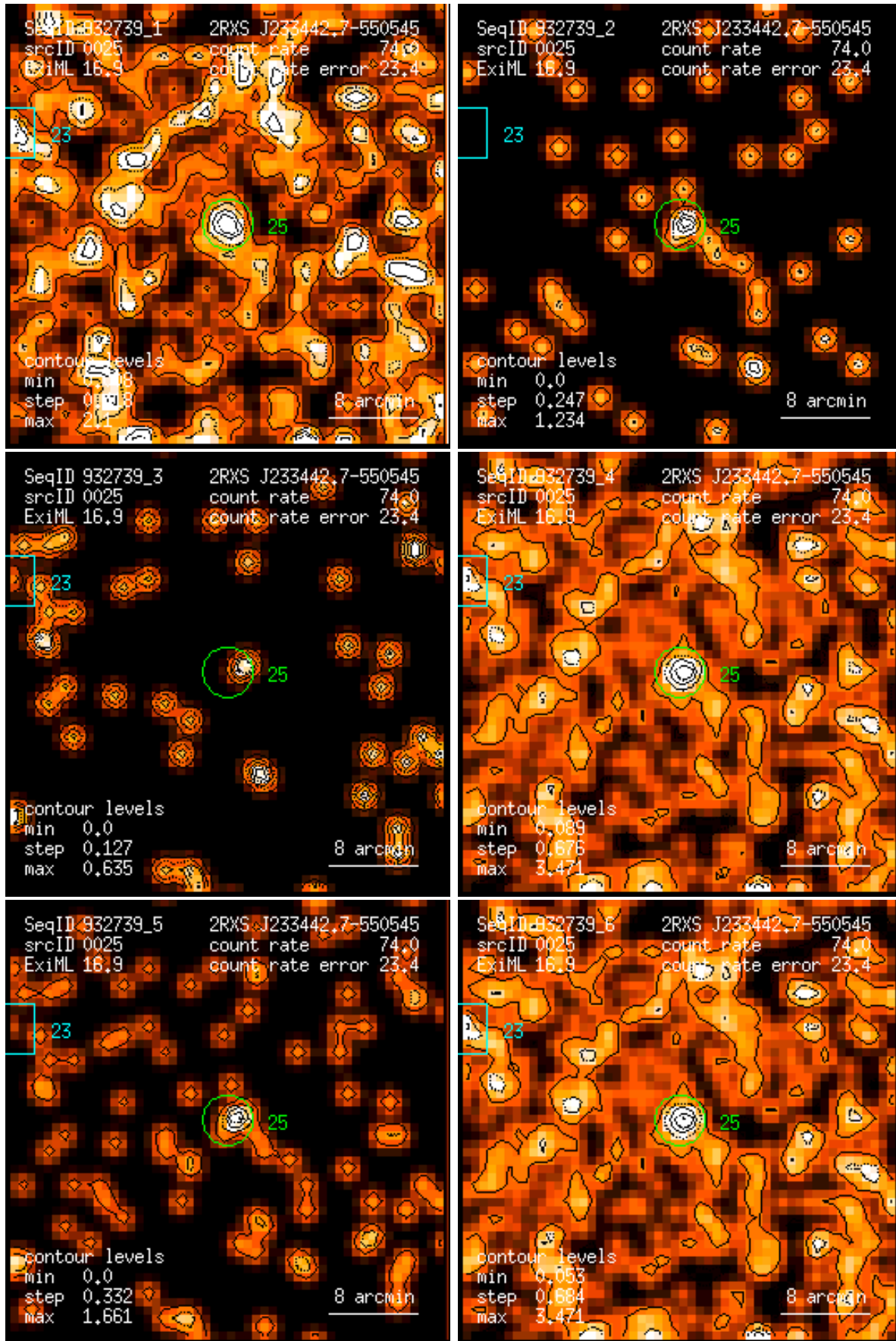
Figure 25: RASS 932739: detection 0025: band rate images, Gaussian filter: (1) PSPC channels 11 – 41, (2) 52 – 90, (3) 91 – 201, (4) 11 – 235, (5) 52 – 201, (6) 11 – 201. Broad band rates in counts/ks. Band rate contour levels in counts/ks/arcmin 2 .
