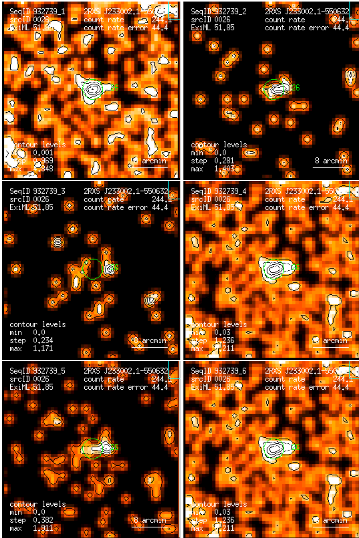
Figure 26: RASS 932739: detection 0026: band rate images, Gaussian filter: (1) PSPC channels 11 – 41, (2) 52 – 90, (3) 91 – 201, (4) 11 – 235, (5) 52 – 201, (6) 11 – 201. Broad band rates in counts/ks. Band rate contour levels in counts/ks/arcmin 2 .
