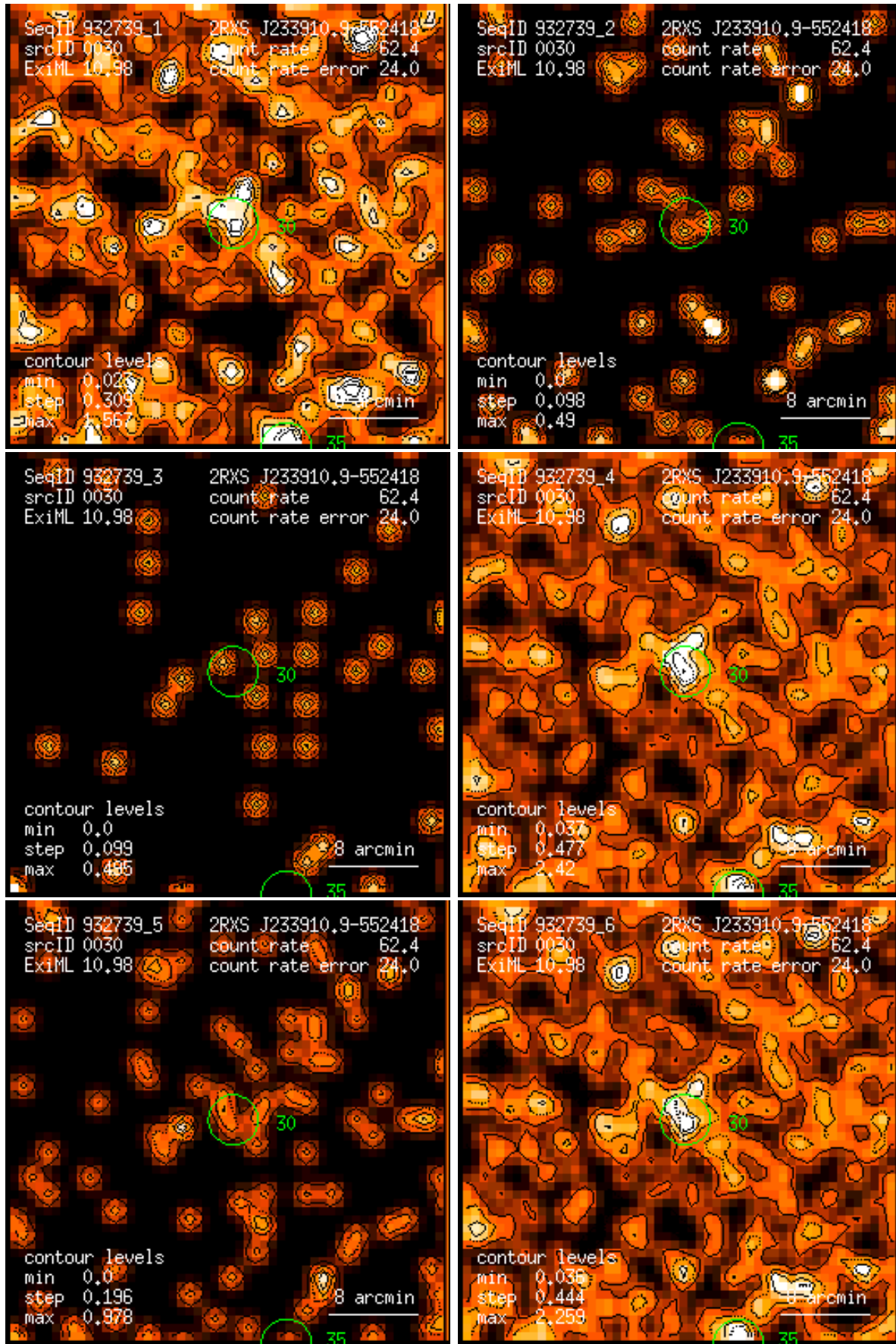
Figure 30: RASS 932739: detection 0030: band rate images, Gaussian filter: (1) PSPC channels 11 – 41, (2) 52 – 90, (3) 91 – 201, (4) 11 – 235, (5) 52 – 201, (6) 11 – 201. Broad band rates in counts/ks. Band rate contour levels in counts/ks/arcmin 2 .
