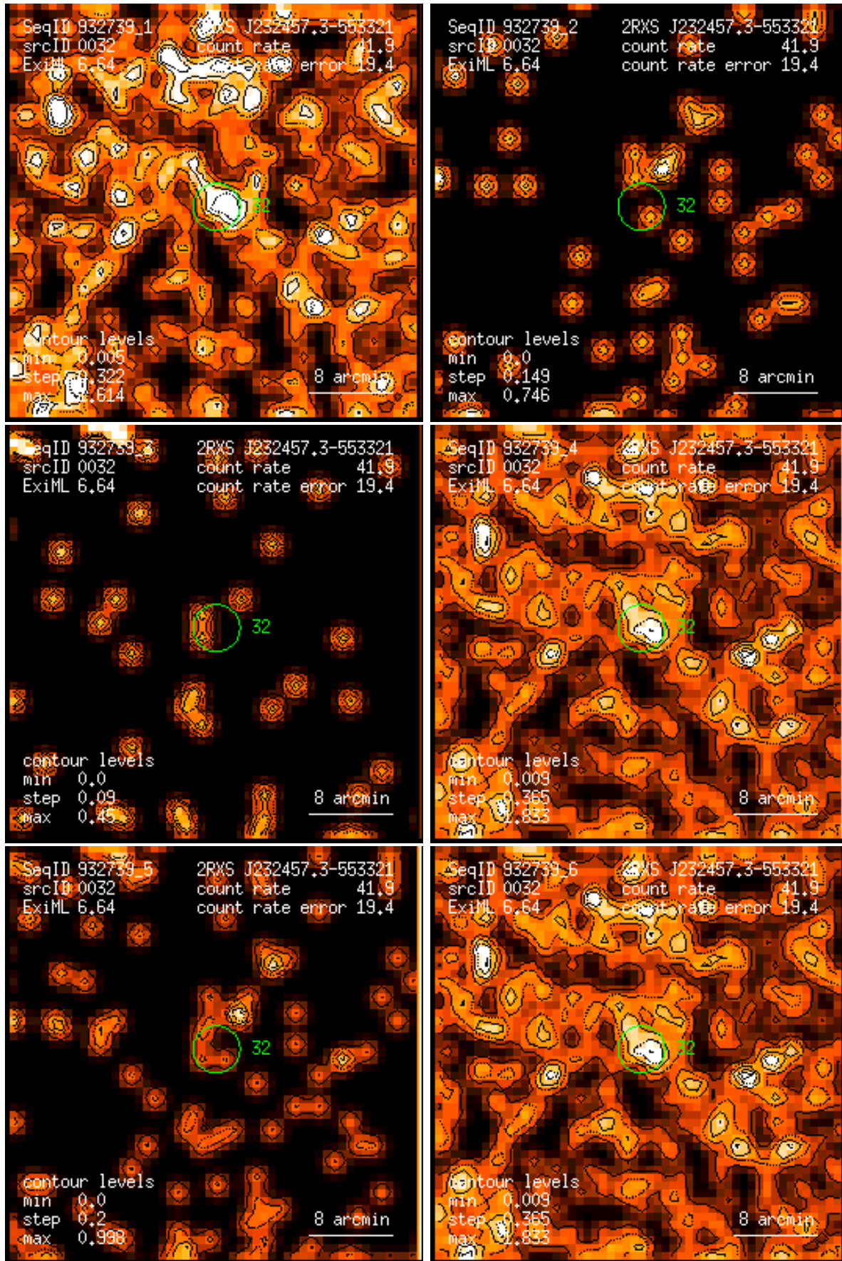
Figure 32: RASS 932739: detection 0032: band rate images, Gaussian filter: (1) PSPC channels 11 – 41, (2) 52 – 90, (3) 91 – 201, (4) 11 – 235, (5) 52 – 201, (6) 11 – 201. Broad band rates in counts/ks. Band rate contour levels in counts/ks/arcmin 2 .
