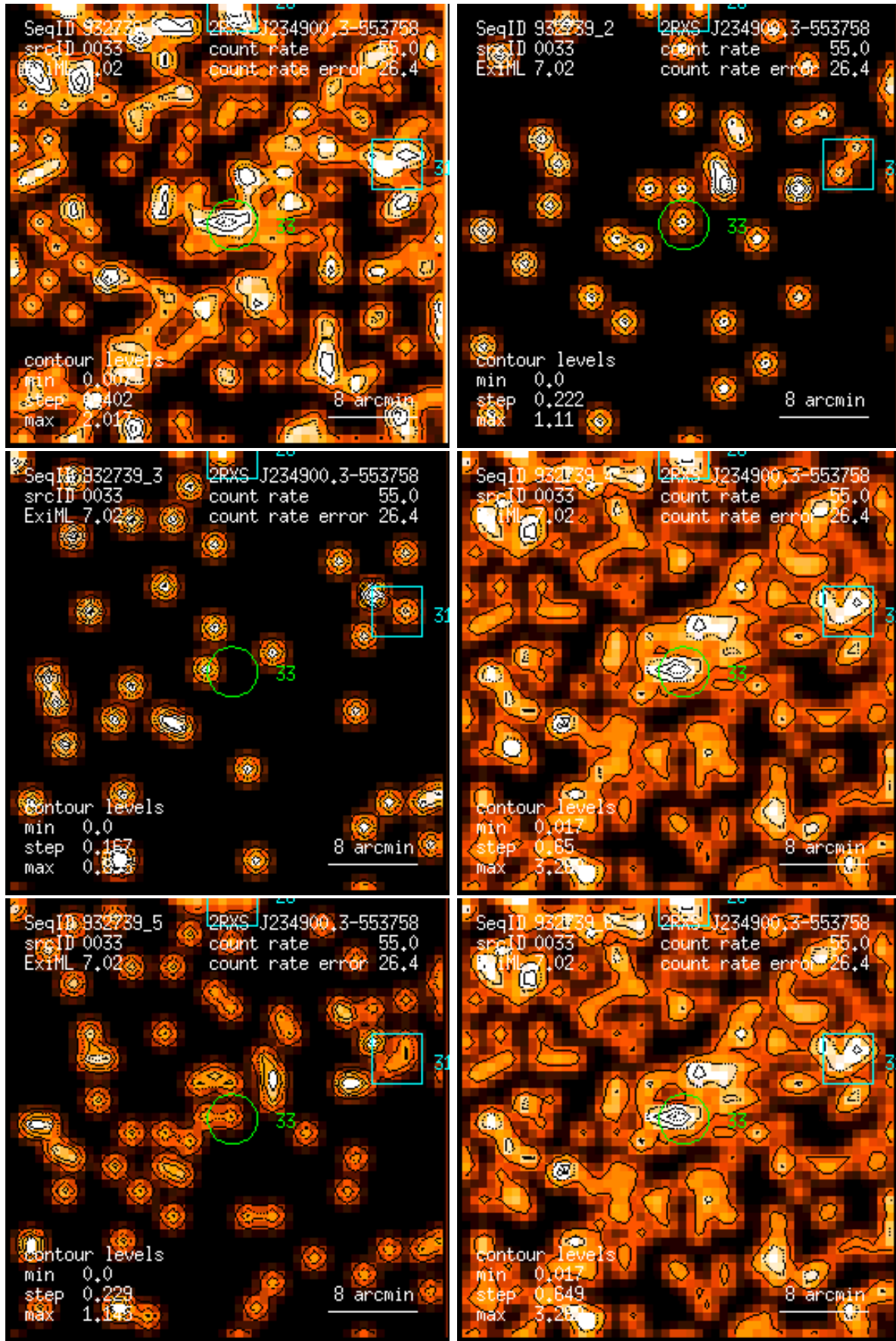
Figure 33: RASS 932739: detection 0033: band rate images, Gaussian filter: (1) PSPC channels 11 – 41, (2) 52 – 90, (3) 91 – 201, (4) 11 – 235, (5) 52 – 201, (6) 11 – 201. Broad band rates in counts/ks. Band rate contour levels in counts/ks/arcmin 2 .
