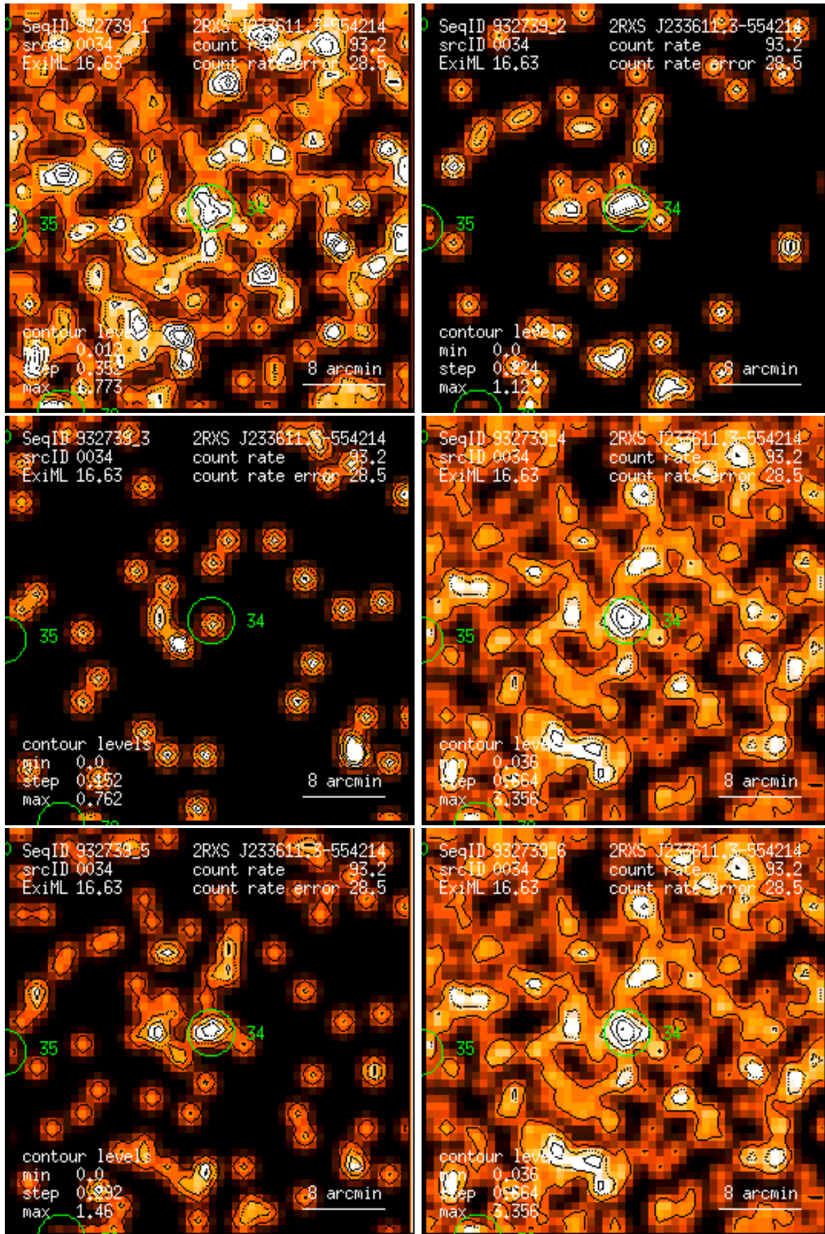
Figure 34: RASS 932739: detection 0034: band rate images, Gaussian filter: (1) PSPC channels 11 – 41, (2) 52 – 90, (3) 91 – 201, (4) 11 – 235, (5) 52 – 201, (6) 11 – 201. Broad band rates in counts/ks. Band rate contour levels in counts/ks/arcmin 2 .
