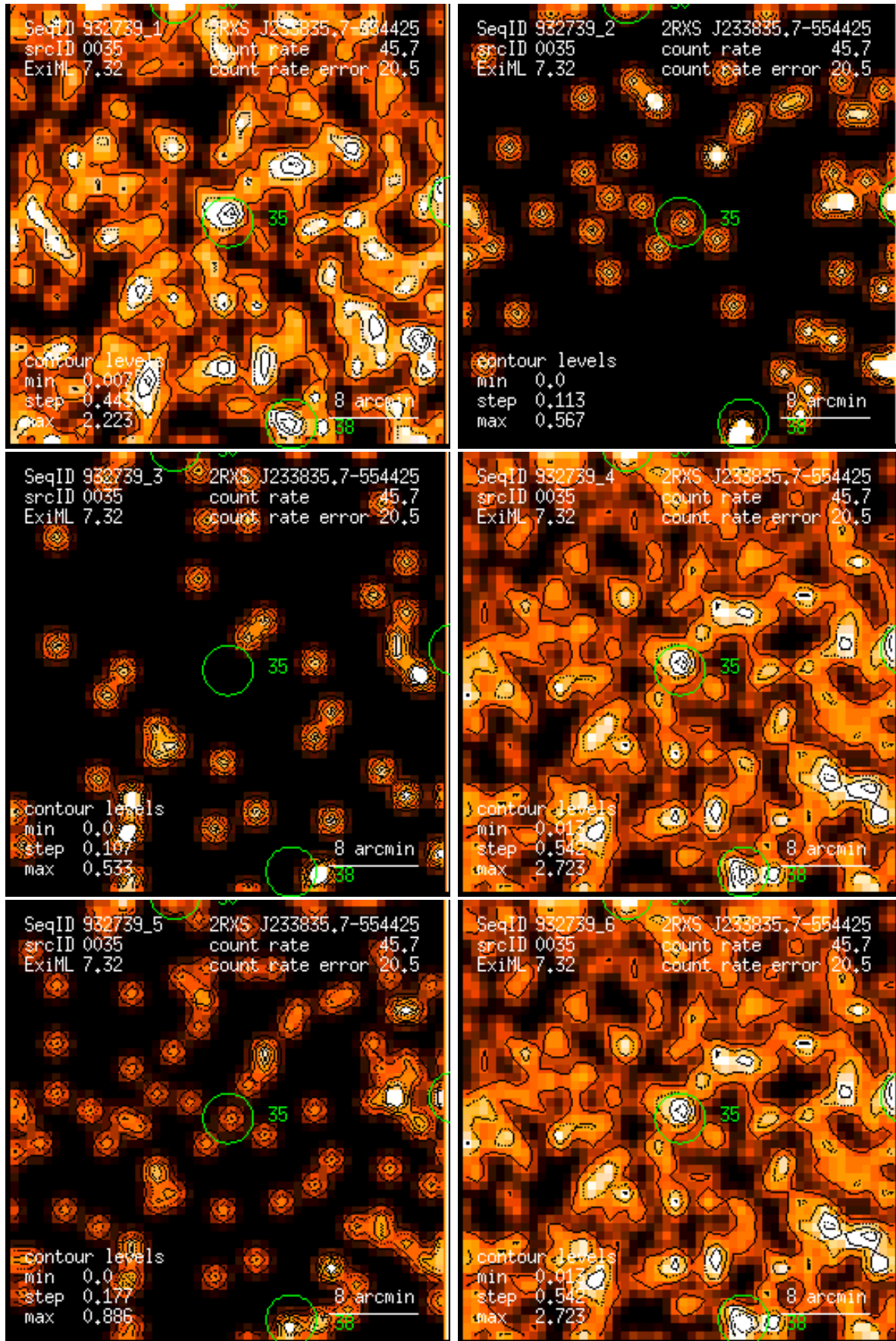
Figure 35: RASS 932739: detection 0035: band rate images, Gaussian filter: (1) PSPC channels 11 – 41, (2) 52 – 90, (3) 91 – 201, (4) 11 – 235, (5) 52 – 201, (6) 11 – 201. Broad band rates in counts/ks. Band rate contour levels in counts/ks/arcmin 2 .
