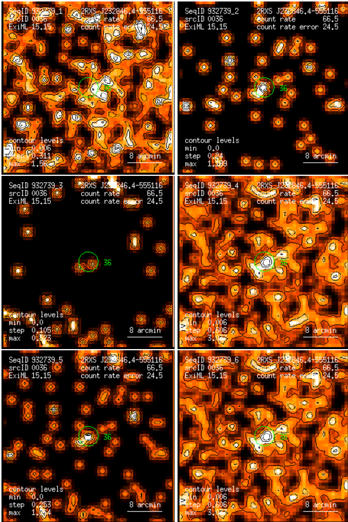
Figure 36: RASS 932739: detection 0036: band rate images, Gaussian filter: (1) PSPC channels 11 – 41, (2) 52 – 90, (3) 91 – 201, (4) 11 – 235, (5) 52 – 201, (6) 11 – 201. Broad band rates in counts/ks. Band rate contour levels in counts/ks/arcmin 2 .
