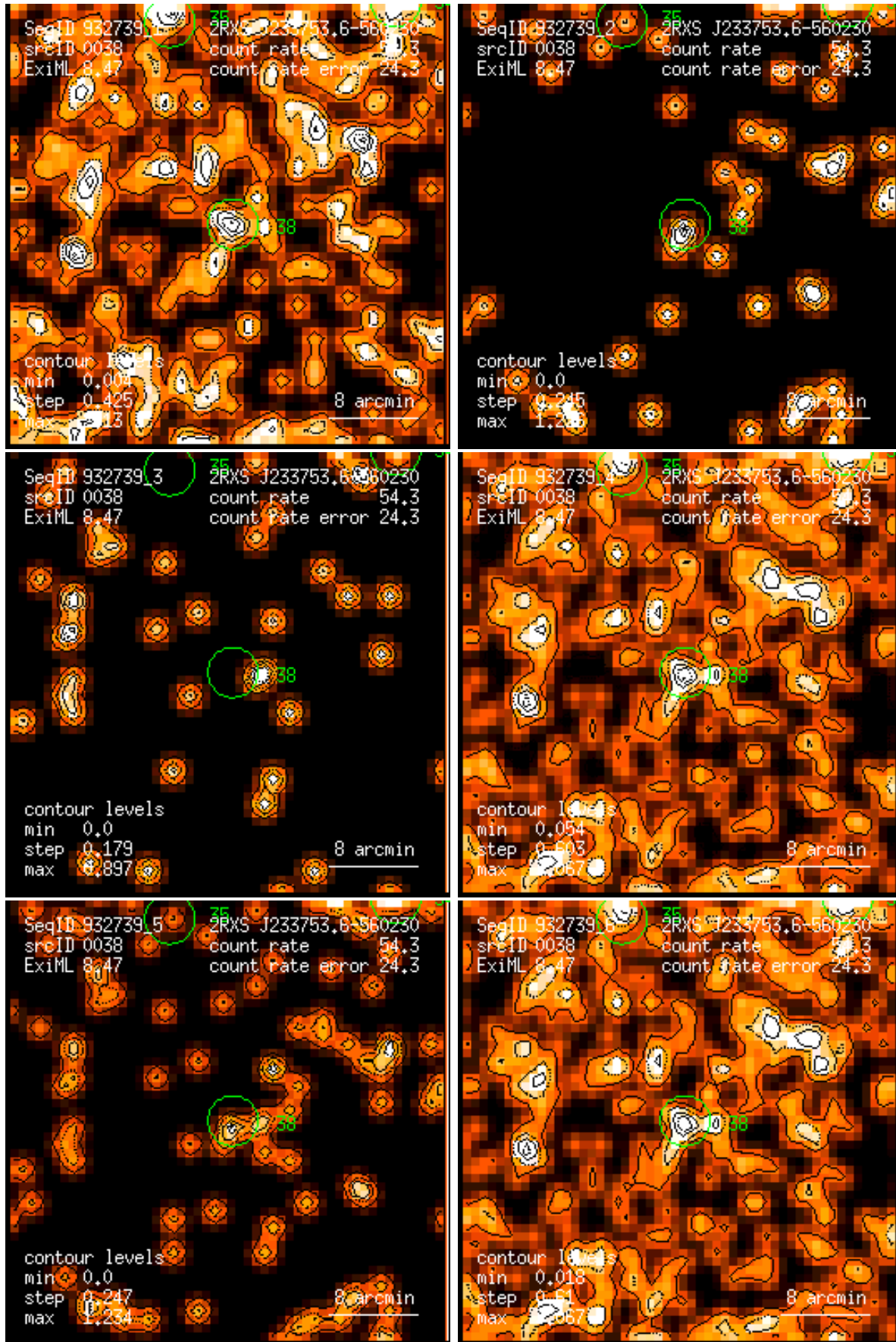
Figure 38: RASS 932739: detection 0038: band rate images, Gaussian filter: (1) PSPC channels 11 – 41, (2) 52 – 90, (3) 91 – 201, (4) 11 – 235, (5) 52 – 201, (6) 11 – 201. Broad band rates in counts/ks. Band rate contour levels in counts/ks/arcmin 2 .
