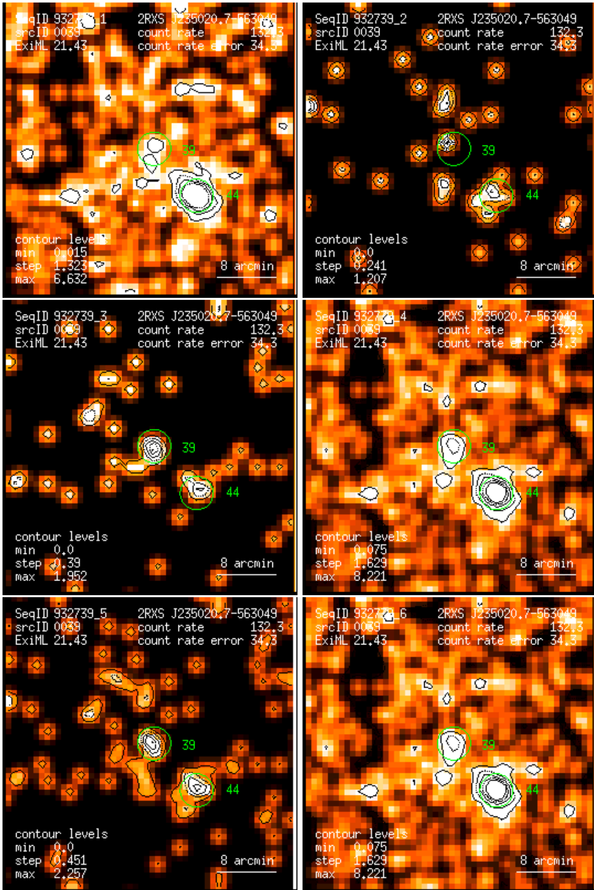
Figure 39: RASS 932739: detection 0039: band rate images, Gaussian filter: (1) PSPC channels 11 – 41, (2) 52 – 90, (3) 91 – 201, (4) 11 – 235, (5) 52 – 201, (6) 11 – 201. Broad band rates in counts/ks. Band rate contour levels in counts/ks/arcmin 2 .
