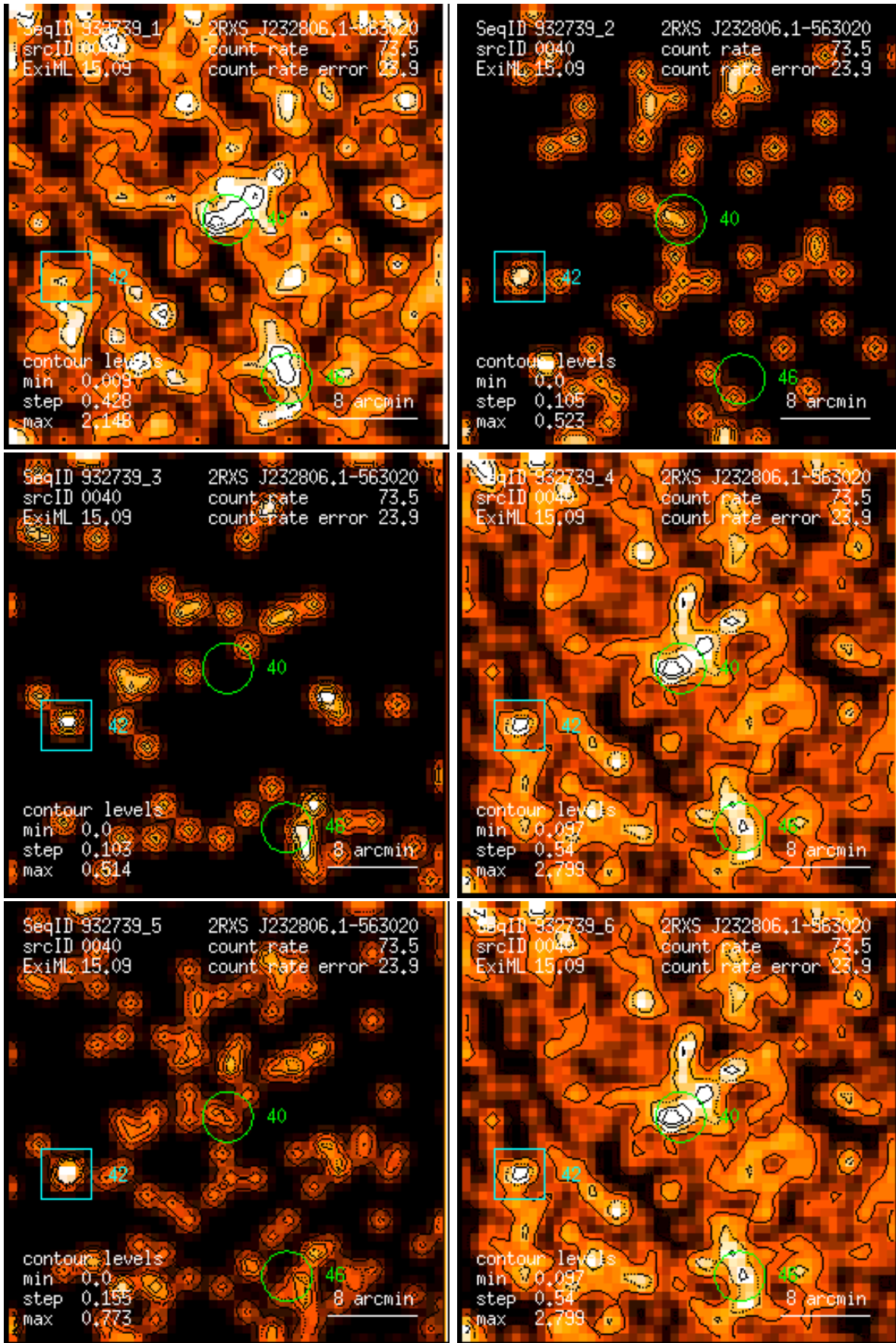
Figure 40: RASS 932739: detection 0040: band rate images, Gaussian filter: (1) PSPC channels 11 – 41, (2) 52 – 90, (3) 91 – 201, (4) 11 – 235, (5) 52 – 201, (6) 11 – 201. Broad band rates in counts/ks. Band rate contour levels in counts/ks/arcmin 2 .
