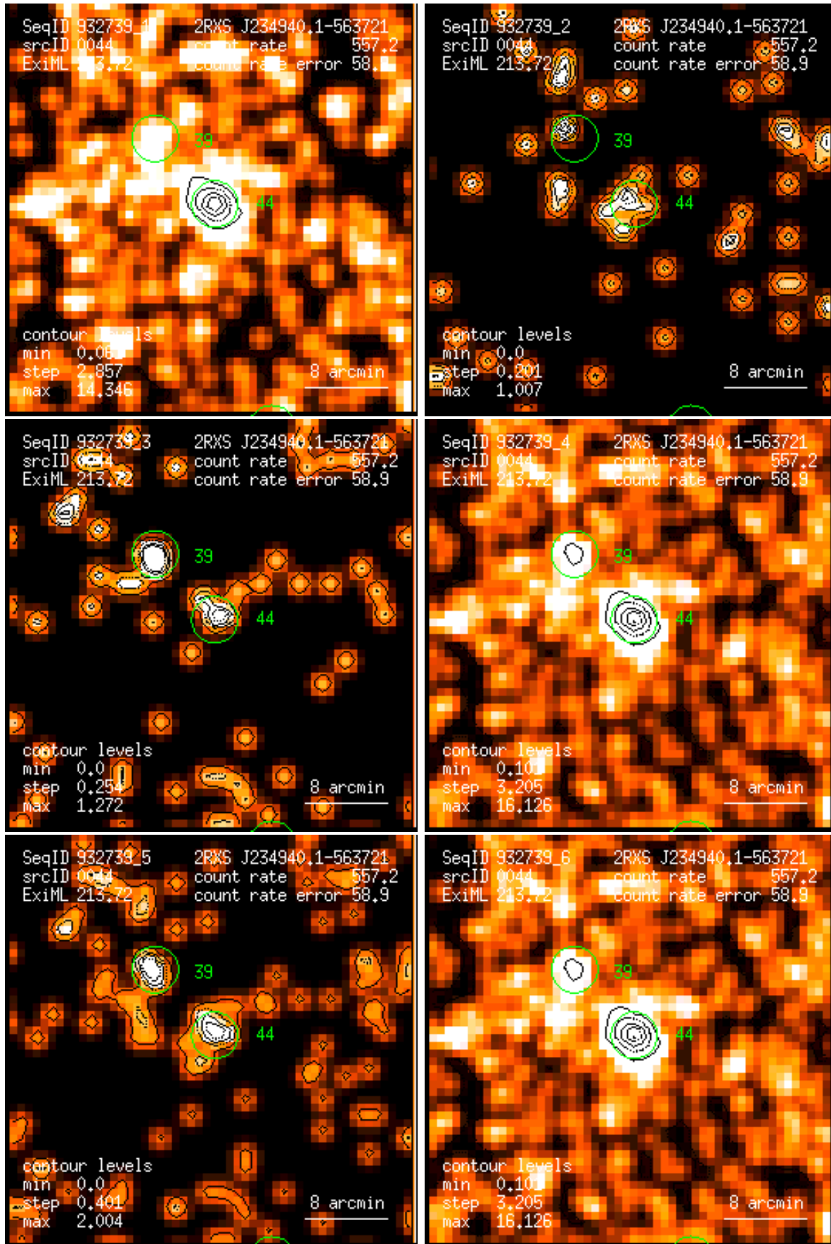
Figure 44: RASS 932739: detection 0044: band rate images, Gaussian filter: (1) PSPC channels 11 – 41, (2) 52 – 90, (3) 91 – 201, (4) 11 – 235, (5) 52 – 201, (6) 11 – 201. Broad band rates in counts/ks. Band rate contour levels in counts/ks/arcmin 2 .
