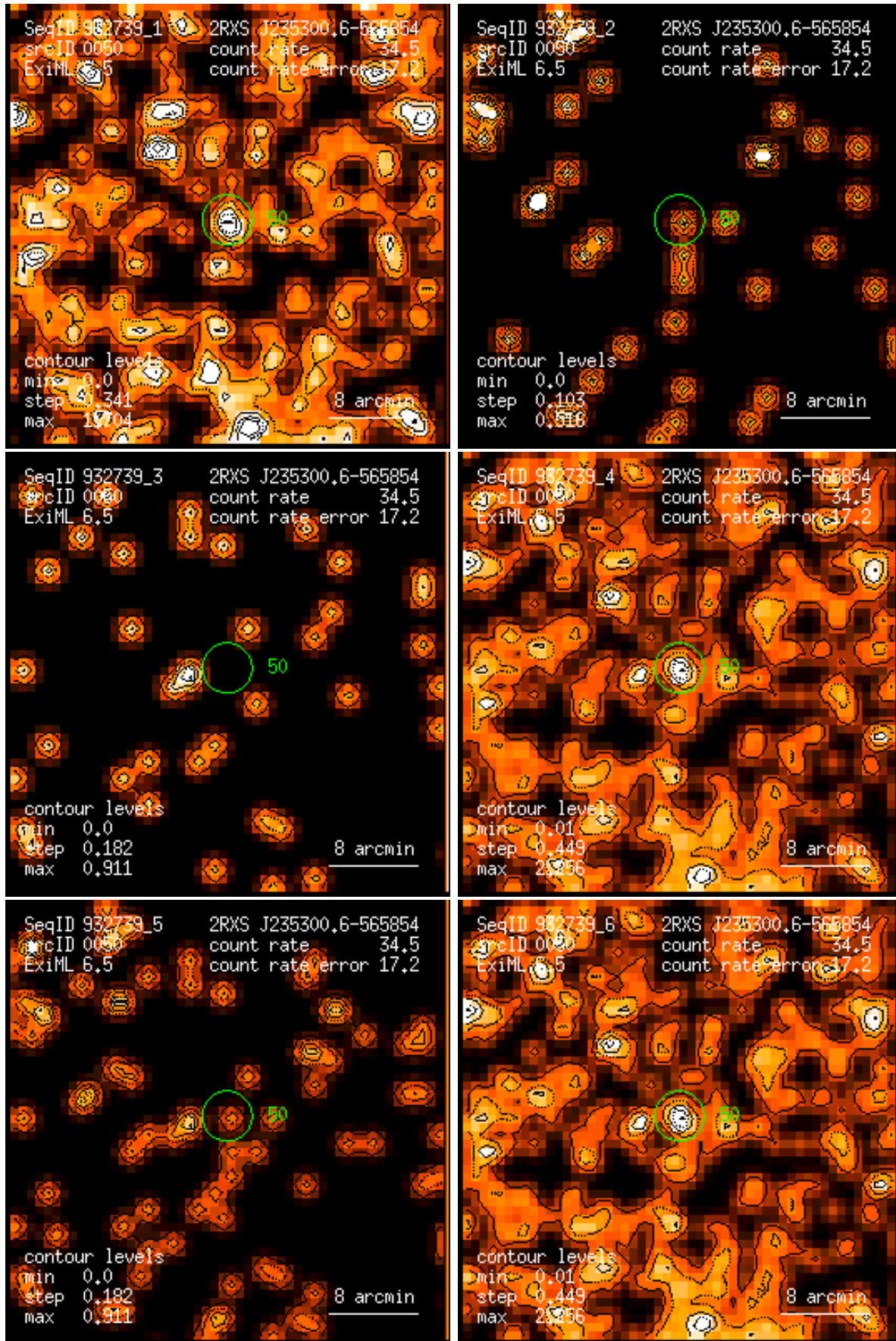
Figure 50: RASS 932739: detection 0050: band rate images, Gaussian filter: (1) PSPC channels 11 – 41, (2) 52 – 90, (3) 91 – 201, (4) 11 – 235, (5) 52 – 201, (6) 11 – 201. Broad band rates in counts/ks. Band rate contour levels in counts/ks/arcmin 2 .
