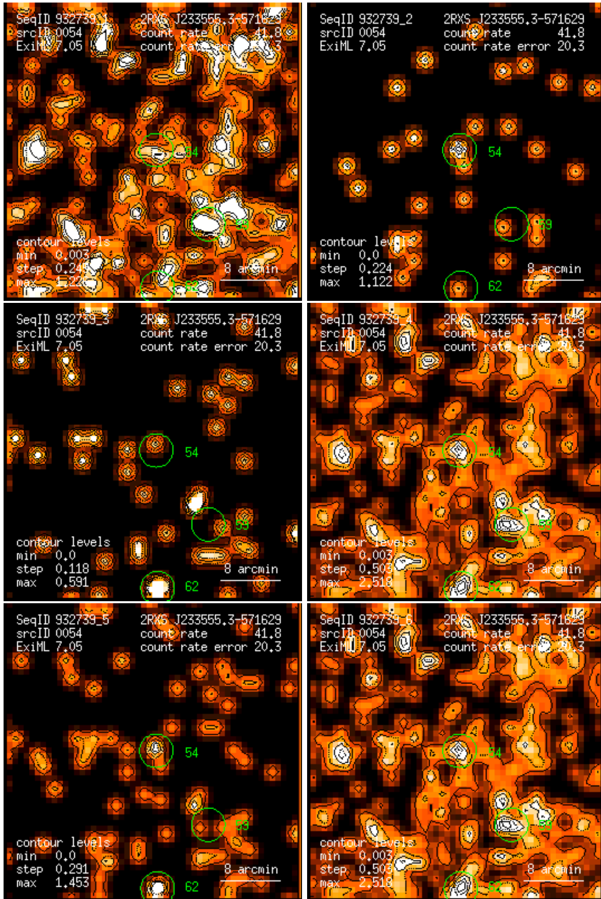
Figure 54: RASS 932739: detection 0054: band rate images, Gaussian filter: (1) PSPC channels 11 – 41, (2) 52 – 90, (3) 91 – 201, (4) 11 – 235, (5) 52 – 201, (6) 11 – 201. Broad band rates in counts/ks. Band rate contour levels in counts/ks/arcmin 2 .
