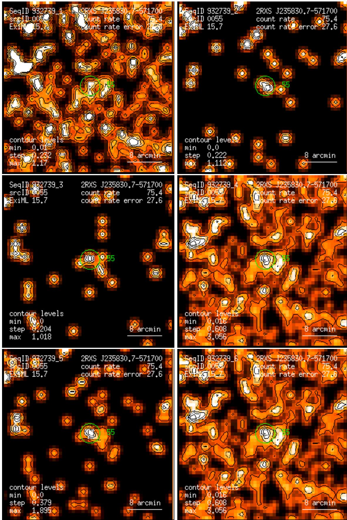
Figure 55: RASS 932739: detection 0055: band rate images, Gaussian filter: (1) PSPC channels 11 – 41, (2) 52 – 90, (3) 91 – 201, (4) 11 – 235, (5) 52 – 201, (6) 11 – 201. Broad band rates in counts/ks. Band rate contour levels in counts/ks/arcmin 2 .
