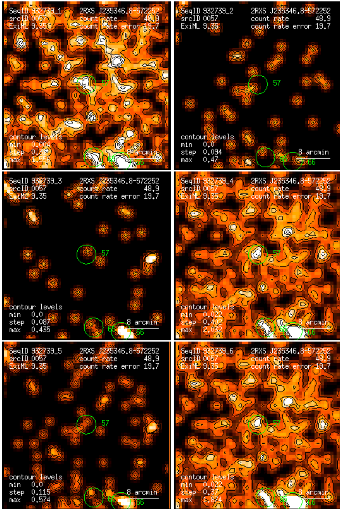
Figure 57: RASS 932739: detection 0057: band rate images, Gaussian filter: (1) PSPC channels 11 – 41, (2) 52 – 90, (3) 91 – 201, (4) 11 – 235, (5) 52 – 201, (6) 11 – 201. Broad band rates in counts/ks. Band rate contour levels in counts/ks/arcmin 2 .
