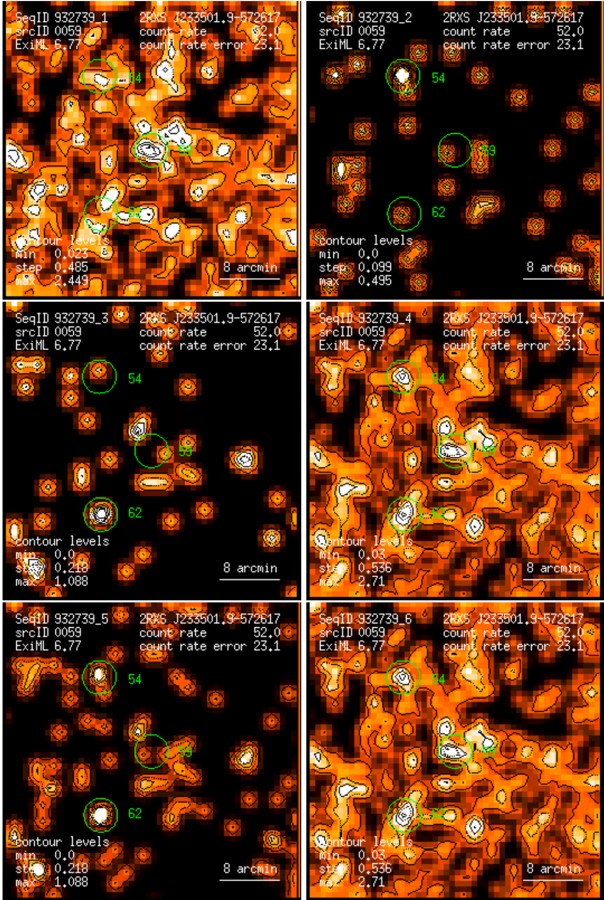
Figure 59: RASS 932739: detection 0059: band rate images, Gaussian filter: (1) PSPC channels 11 – 41, (2) 52 – 90, (3) 91 – 201, (4) 11 – 235, (5) 52 – 201, (6) 11 – 201. Broad band rates in counts/ks. Band rate contour levels in counts/ks/arcmin 2 .
