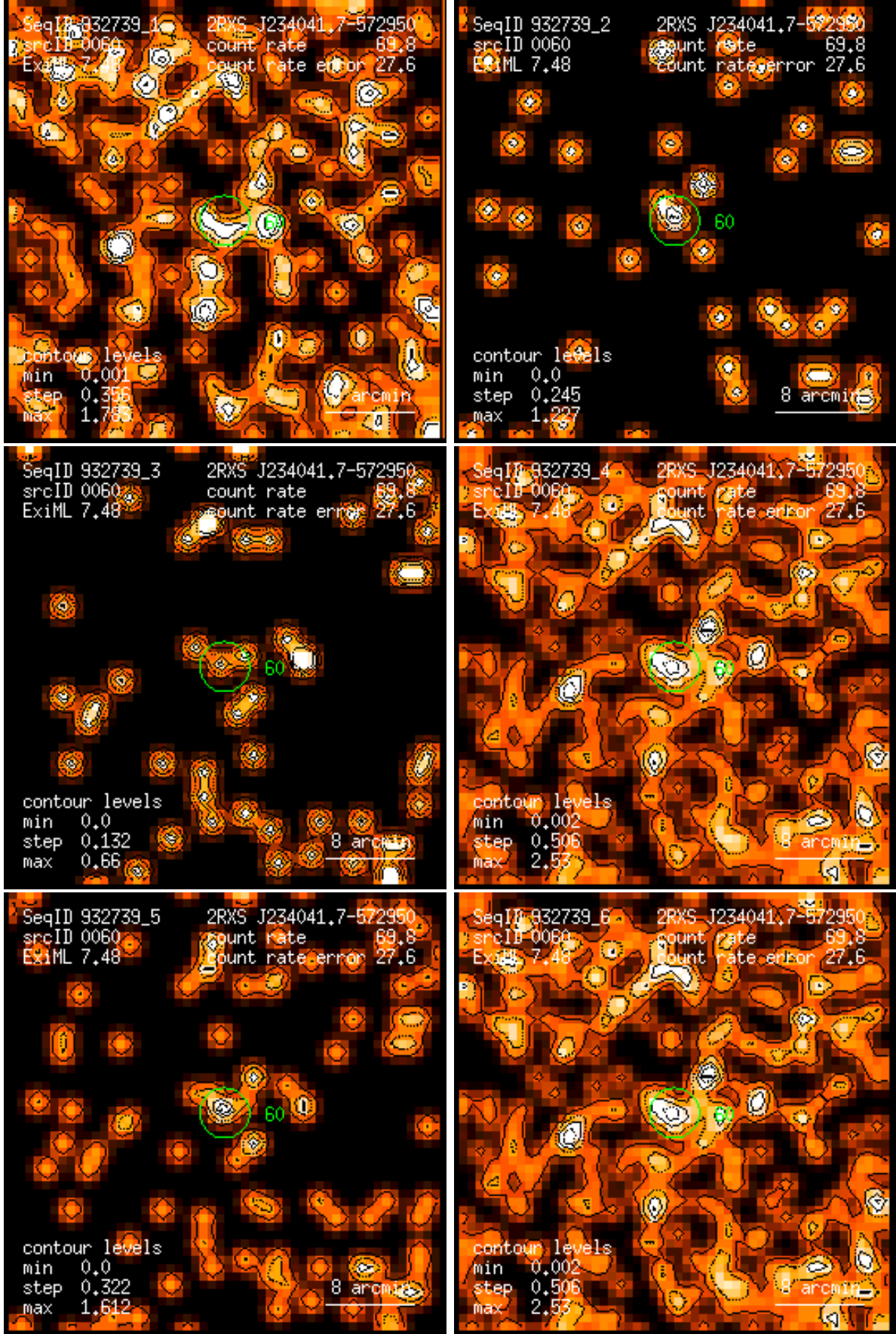
Figure 60: RASS 932739: detection 0060: band rate images, Gaussian filter: (1) PSPC channels 11 – 41, (2) 52 – 90, (3) 91 – 201, (4) 11 – 235, (5) 52 – 201, (6) 11 – 201. Broad band rates in counts/ks. Band rate contour levels in counts/ks/arcmin 2 .
