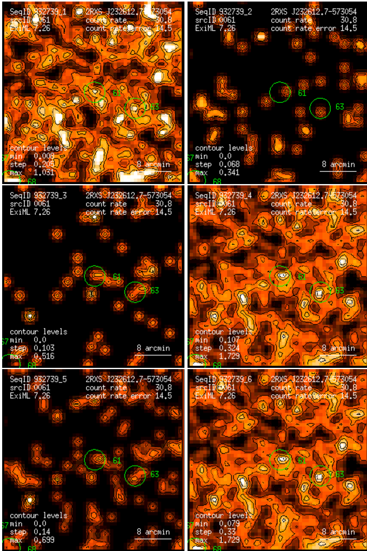
Figure 61: RASS 932739: detection 0061: band rate images, Gaussian filter: (1) PSPC channels 11 – 41, (2) 52 – 90, (3) 91 – 201, (4) 11 – 235, (5) 52 – 201, (6) 11 – 201. Broad band rates in counts/ks. Band rate contour levels in counts/ks/arcmin 2 .
