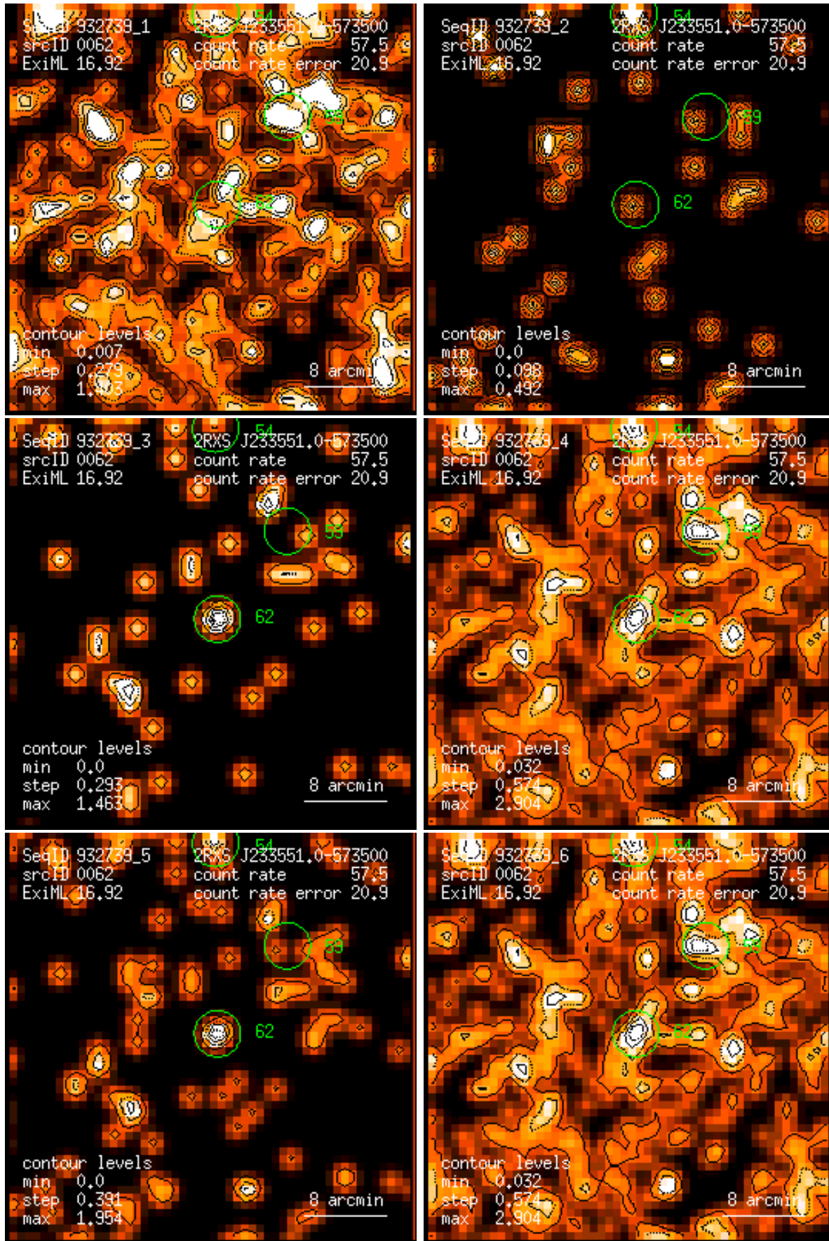
Figure 62: RASS 932739: detection 0062: band rate images, Gaussian filter: (1) PSPC channels 11 – 41, (2) 52 – 90, (3) 91 – 201, (4) 11 – 235, (5) 52 – 201, (6) 11 – 201. Broad band rates in counts/ks. Band rate contour levels in counts/ks/arcmin 2 .
