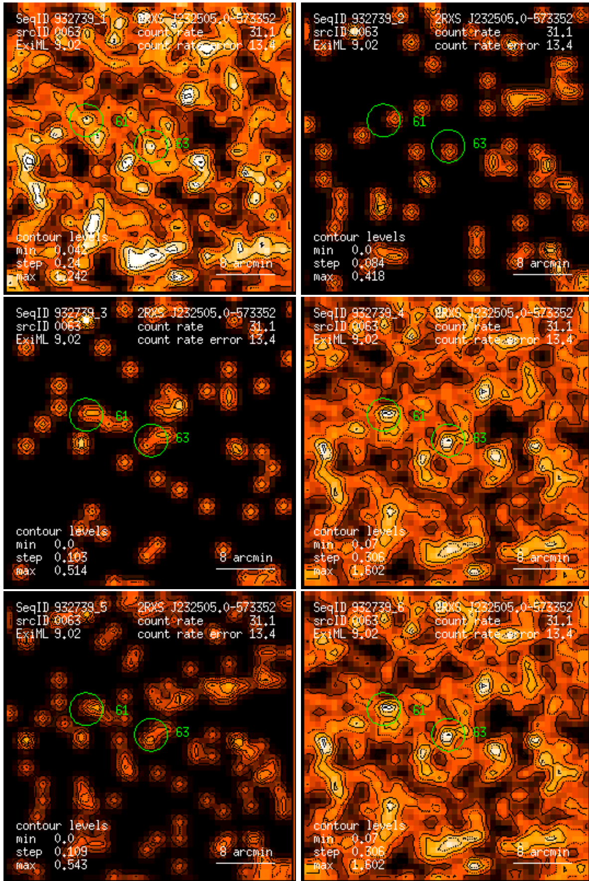
Figure 63: RASS 932739: detection 0063: band rate images, Gaussian filter: (1) PSPC channels 11 – 41, (2) 52 – 90, (3) 91 – 201, (4) 11 – 235, (5) 52 – 201, (6) 11 – 201. Broad band rates in counts/ks. Band rate contour levels in counts/ks/arcmin 2 .
