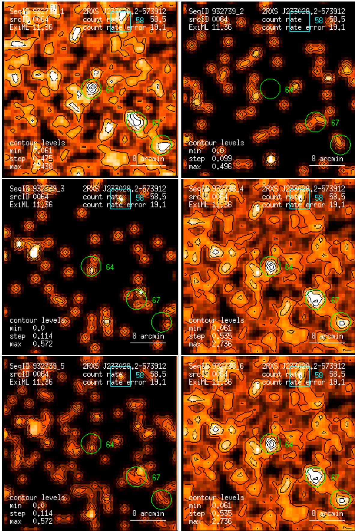
Figure 64: RASS 932739: detection 0064: band rate images, Gaussian filter: (1) PSPC channels 11 – 41, (2) 52 – 90, (3) 91 – 201, (4) 11 – 235, (5) 52 – 201, (6) 11 – 201. Broad band rates in counts/ks. Band rate contour levels in counts/ks/arcmin 2 .
