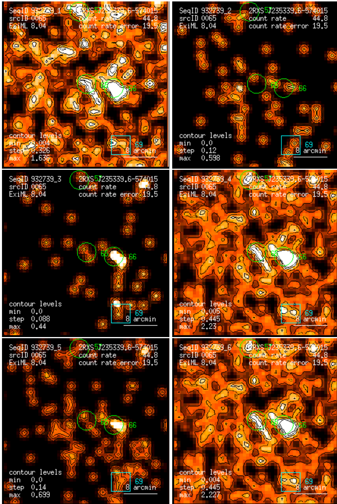
Figure 65: RASS 932739: detection 0065: band rate images, Gaussian filter: (1) PSPC channels 11 – 41, (2) 52 – 90, (3) 91 – 201, (4) 11 – 235, (5) 52 – 201, (6) 11 – 201. Broad band rates in counts/ks. Band rate contour levels in counts/ks/arcmin 2 .
