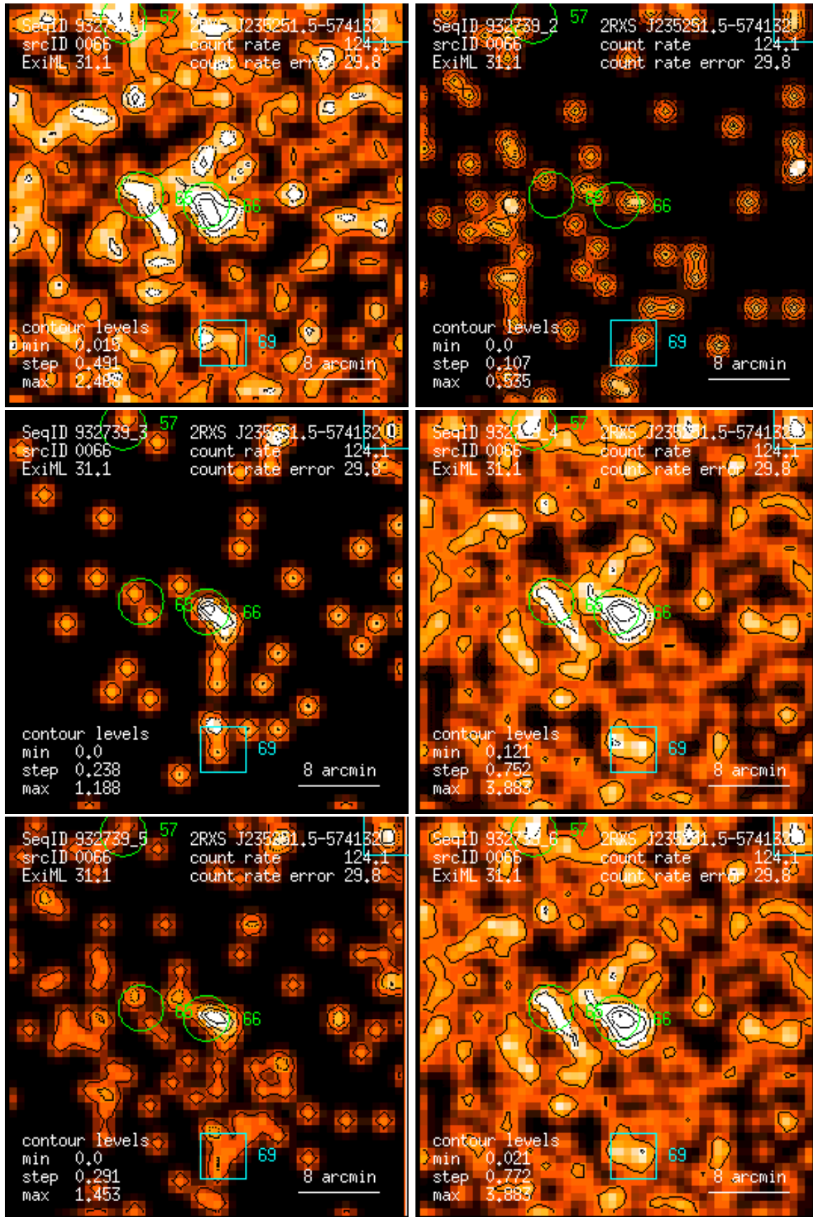
Figure 66: RASS 932739: detection 0066: band rate images, Gaussian filter: (1) PSPC channels 11 – 41, (2) 52 – 90, (3) 91 – 201, (4) 11 – 235, (5) 52 – 201, (6) 11 – 201. Broad band rates in counts/ks. Band rate contour levels in counts/ks/arcmin 2 .
