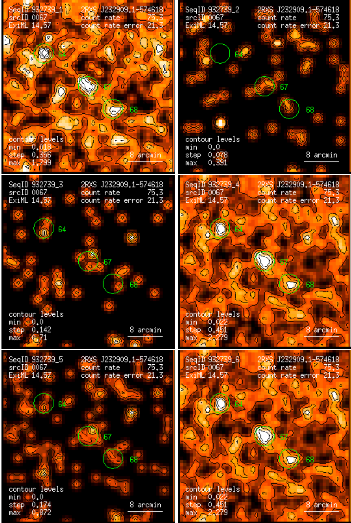
Figure 67: RASS 932739: detection 0067: band rate images, Gaussian filter: (1) PSPC channels 11 – 41, (2) 52 – 90, (3) 91 – 201, (4) 11 – 235, (5) 52 – 201, (6) 11 – 201. Broad band rates in counts/ks. Band rate contour levels in counts/ks/arcmin 2 .
