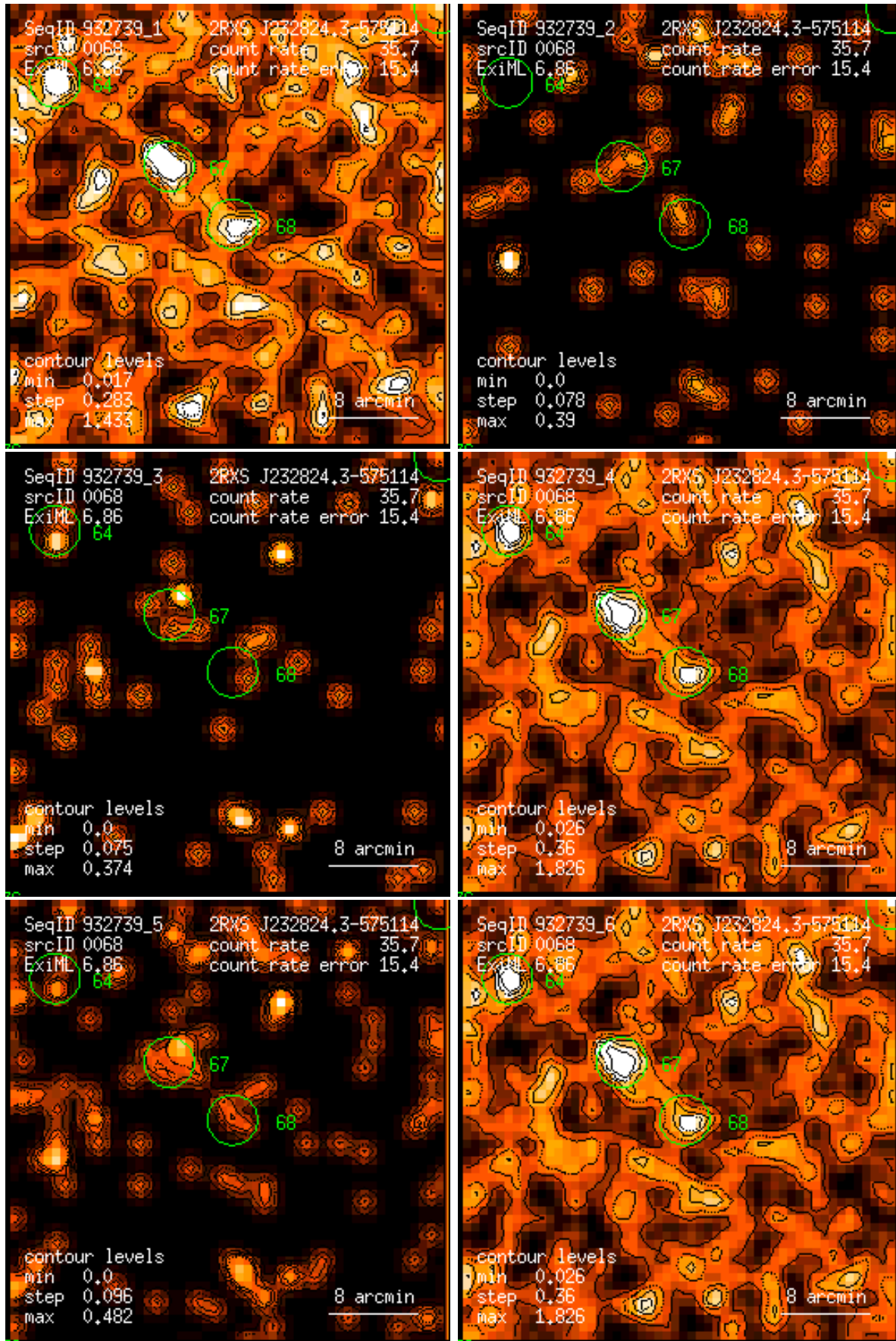
Figure 68: RASS 932739: detection 0068: band rate images, Gaussian filter: (1) PSPC channels 11 – 41, (2) 52 – 90, (3) 91 – 201, (4) 11 – 235, (5) 52 – 201, (6) 11 – 201. Broad band rates in counts/ks. Band rate contour levels in counts/ks/arcmin 2 .
