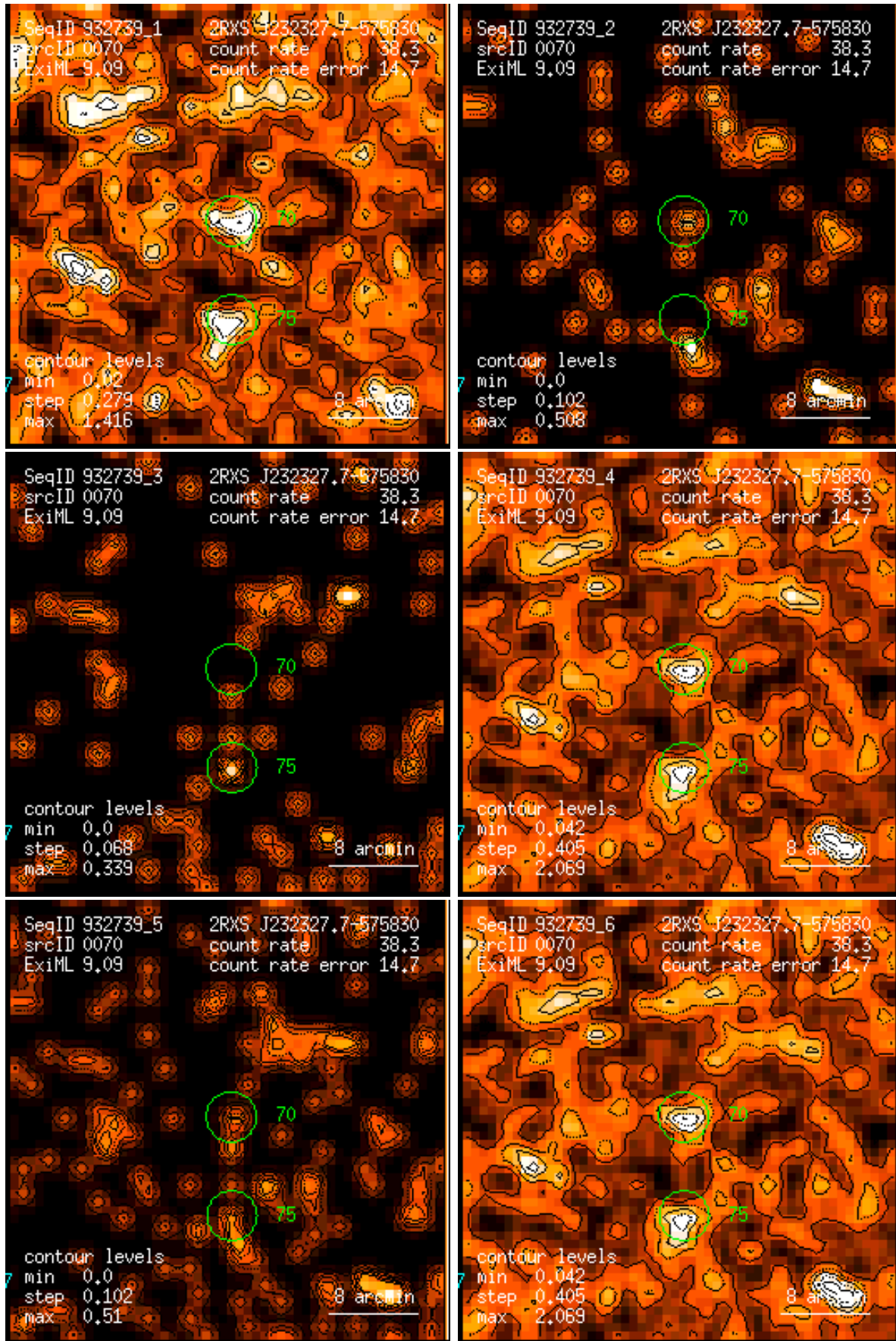
Figure 70: RASS 932739: detection 0070: band rate images, Gaussian filter: (1) PSPC channels 11 – 41, (2) 52 – 90, (3) 91 – 201, (4) 11 – 235, (5) 52 – 201, (6) 11 – 201. Broad band rates in counts/ks. Band rate contour levels in counts/ks/arcmin 2 .
