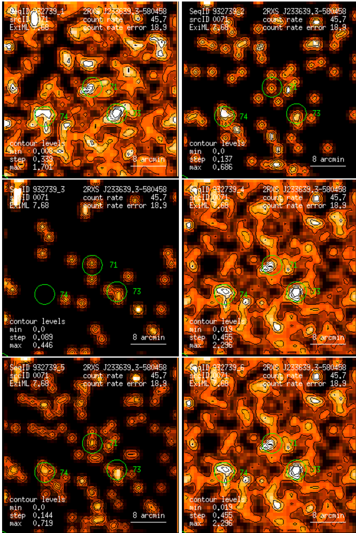
Figure 71: RASS 932739: detection 0071: band rate images, Gaussian filter: (1) PSPC channels 11 – 41, (2) 52 – 90, (3) 91 – 201, (4) 11 – 235, (5) 52 – 201, (6) 11 – 201. Broad band rates in counts/ks. Band rate contour levels in counts/ks/arcmin 2 .
