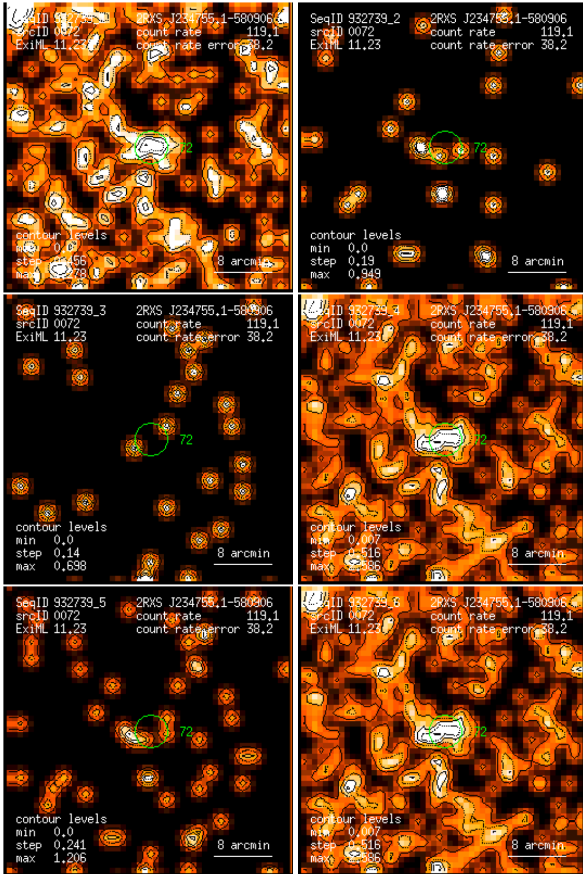
Figure 72: RASS 932739: detection 0072: band rate images, Gaussian filter: (1) PSPC channels 11 – 41, (2) 52 – 90, (3) 91 – 201, (4) 11 – 235, (5) 52 – 201, (6) 11 – 201. Broad band rates in counts/ks. Band rate contour levels in counts/ks/arcmin 2 .
