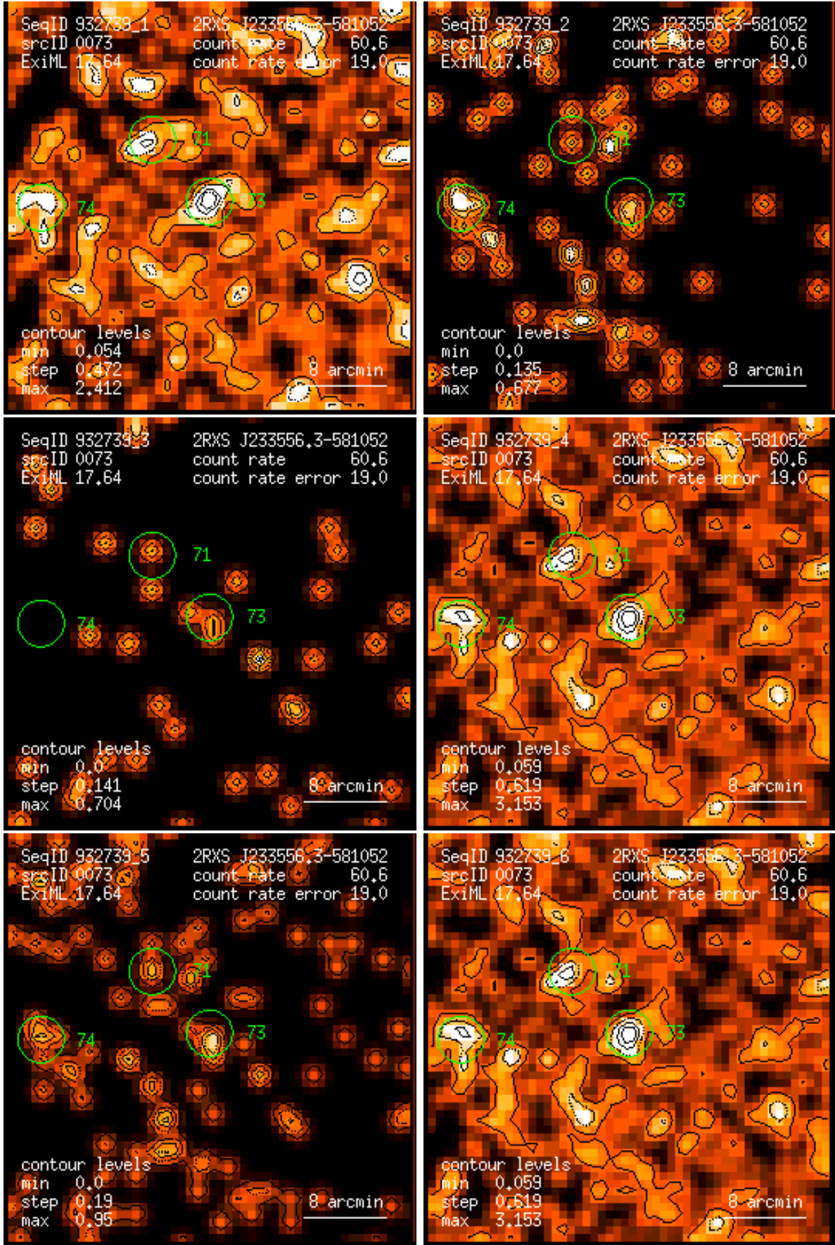
Figure 73: RASS 932739: detection 0073: band rate images, Gaussian filter: (1) PSPC channels 11 – 41, (2) 52 – 90, (3) 91 – 201, (4) 11 – 235, (5) 52 – 201, (6) 11 – 201. Broad band rates in counts/ks. Band rate contour levels in counts/ks/arcmin 2 .
