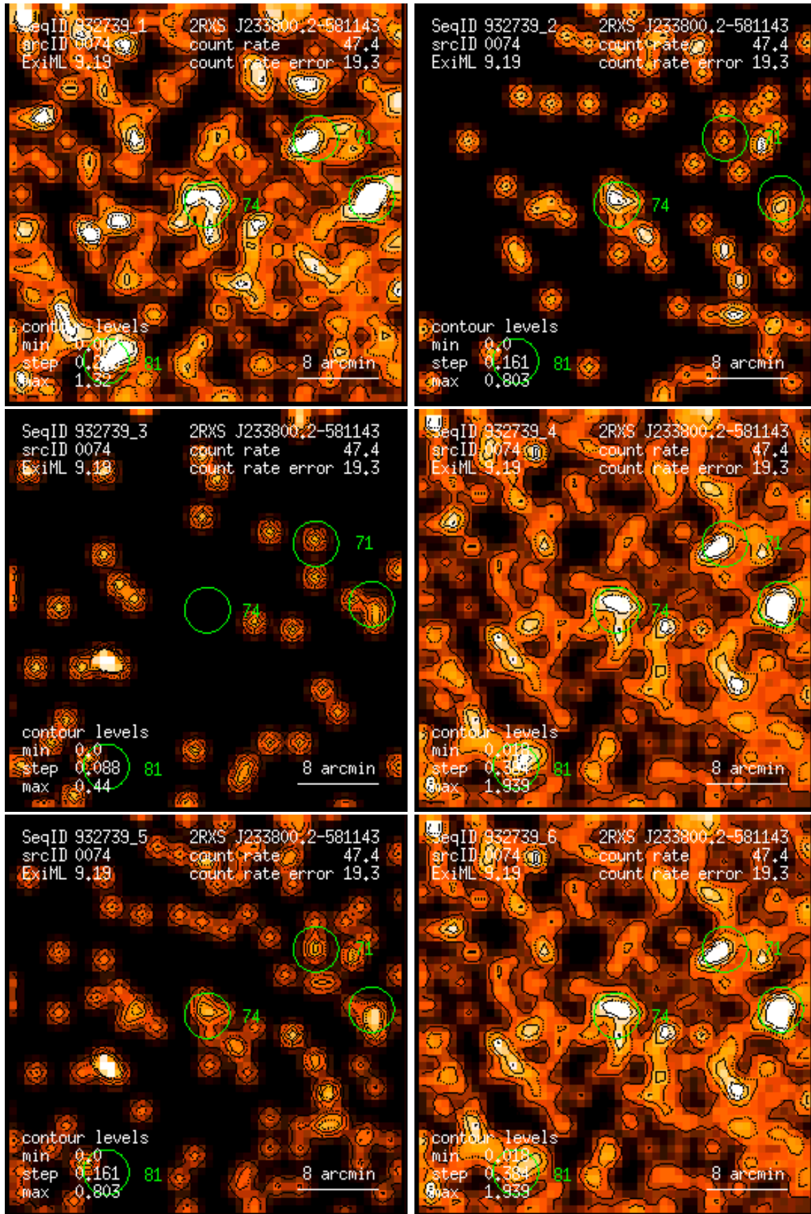
Figure 74: RASS 932739: detection 0074: band rate images, Gaussian filter: (1) PSPC channels 11 – 41, (2) 52 – 90, (3) 91 – 201, (4) 11 – 235, (5) 52 – 201, (6) 11 – 201. Broad band rates in counts/ks. Band rate contour levels in counts/ks/arcmin 2 .
