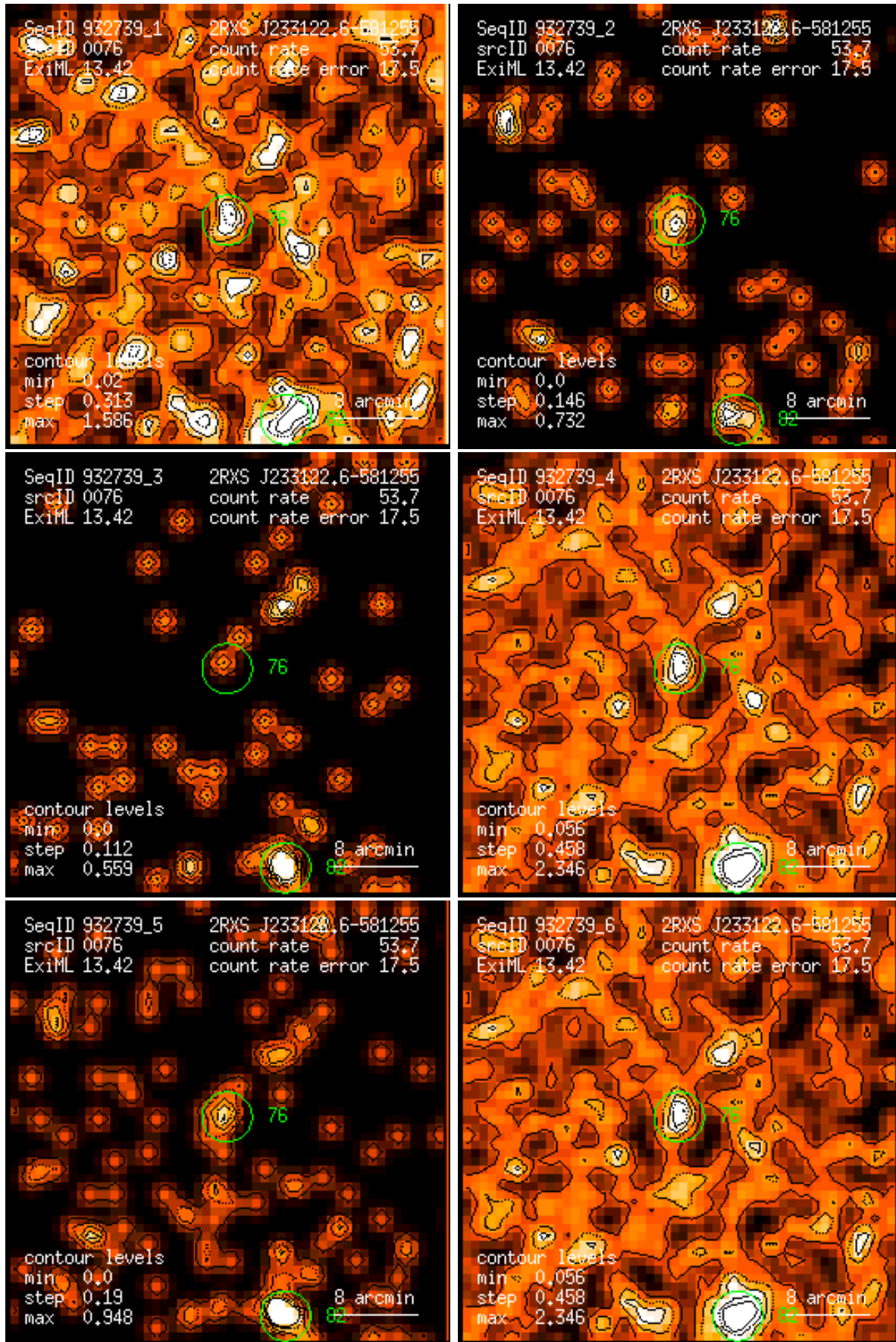
Figure 76: RASS 932739: detection 0076: band rate images, Gaussian filter: (1) PSPC channels 11 – 41, (2) 52 – 90, (3) 91 – 201, (4) 11 – 235, (5) 52 – 201, (6) 11 – 201. Broad band rates in counts/ks. Band rate contour levels in counts/ks/arcmin 2 .
