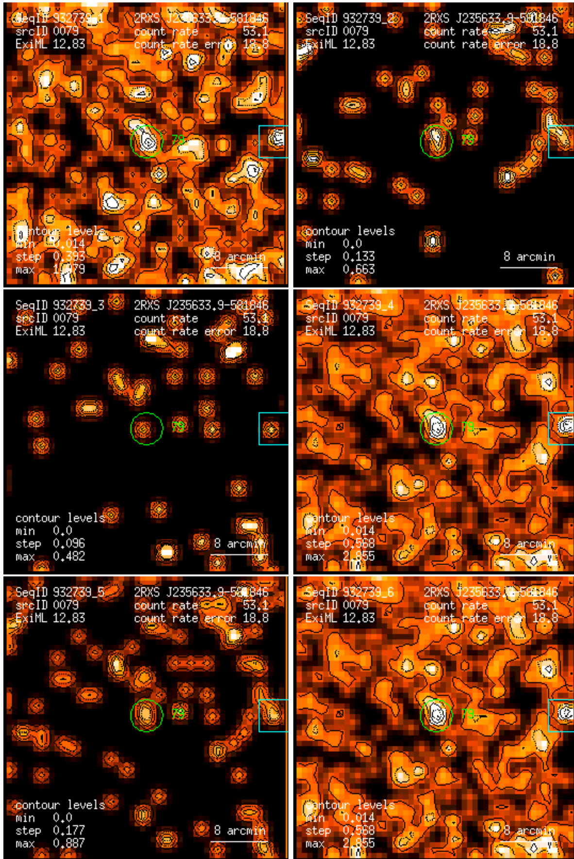
Figure 79: RASS 932739: detection 0079: band rate images, Gaussian filter: (1) PSPC channels 11 – 41, (2) 52 – 90, (3) 91 – 201, (4) 11 – 235, (5) 52 – 201, (6) 11 – 201. Broad band rates in counts/ks. Band rate contour levels in counts/ks/arcmin 2 .
